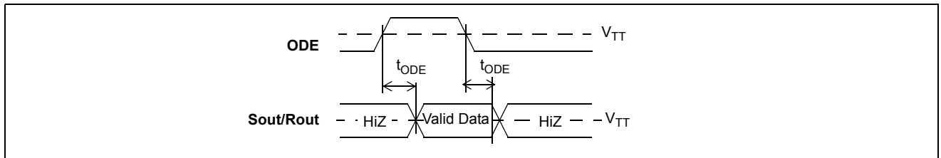
Figure 11 - Output Driver Enable (ODE)
