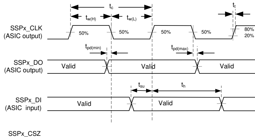
Figure 6-11. Synchronous Serial Port Interface – Slave (Modes 0/3)
