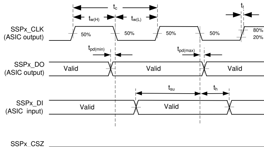
Figure 6-10. Synchronous Serial Port Interface – Master (Modes 0/3)
