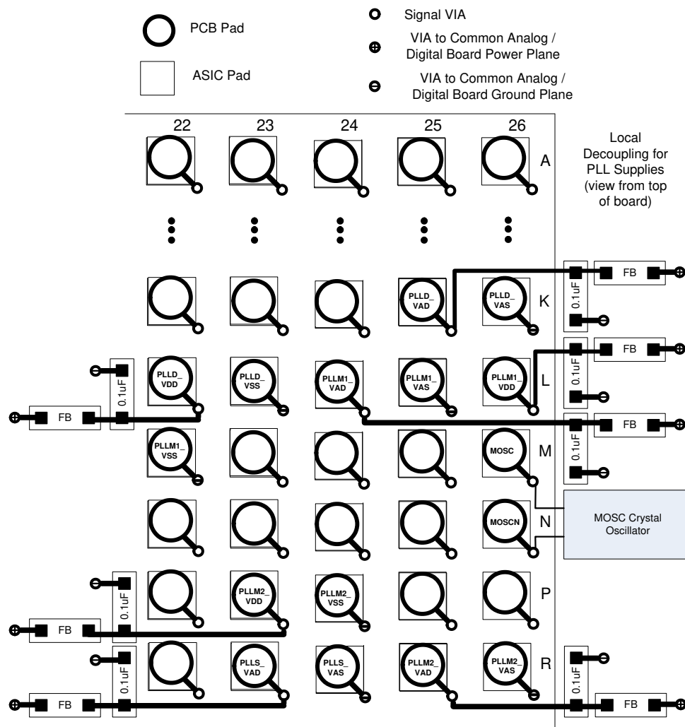
Figure 10-3. High Frequency Decoupling
