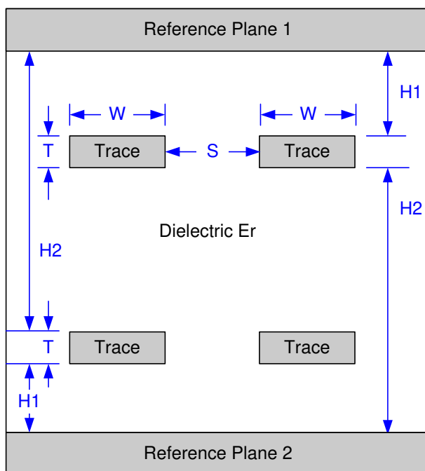
Figure 10-5. PCB Stackup Geometries
