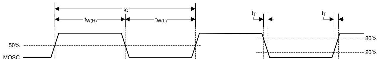
Figure 6-1. System Oscillators
