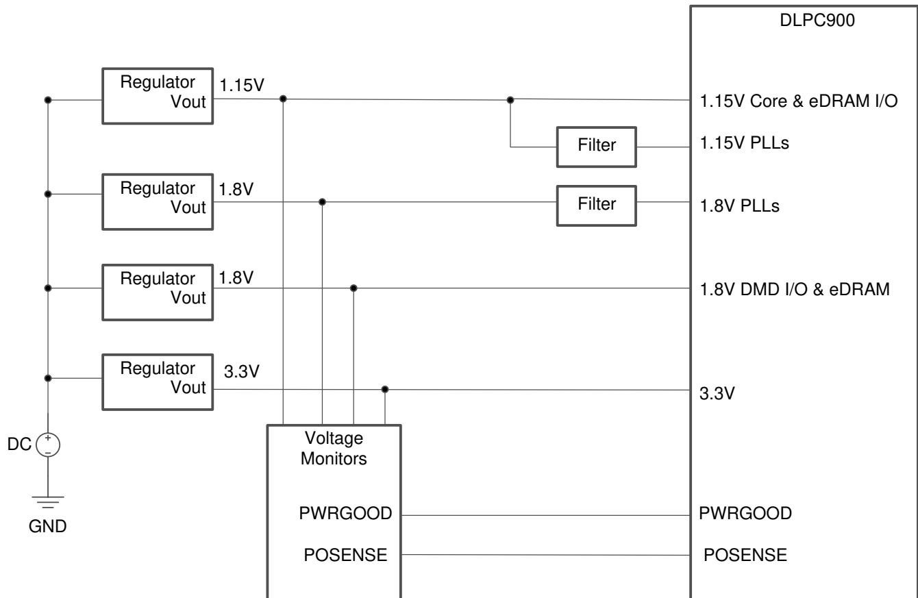
Figure 9-1. Power Regulation
