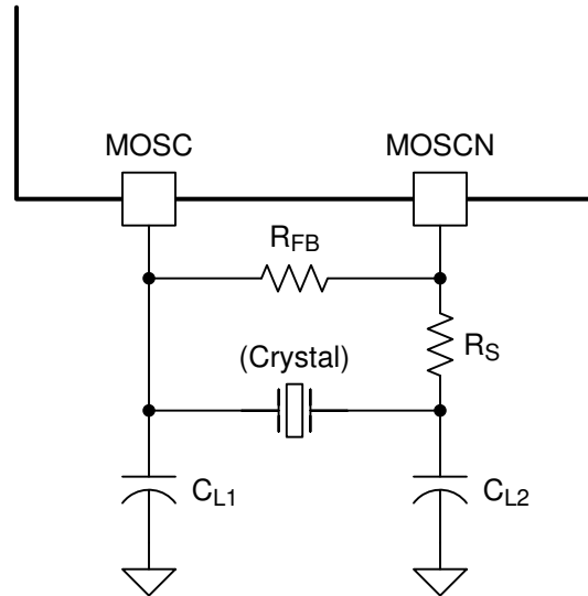
Figure 10-4. Crystal Oscillator Configuration
