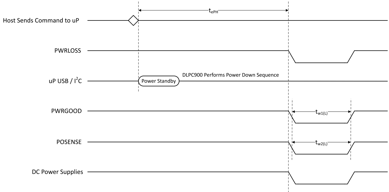
Figure 6-4. Anticipated Power Down Timing Diagram
