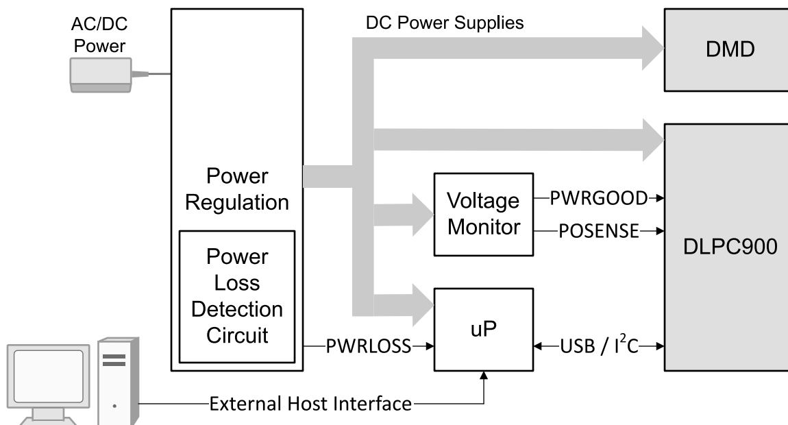
Figure 6-3. Power Distribution Layout Example
