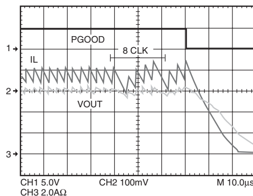
Figure 7. Over-Current protection waveforms
