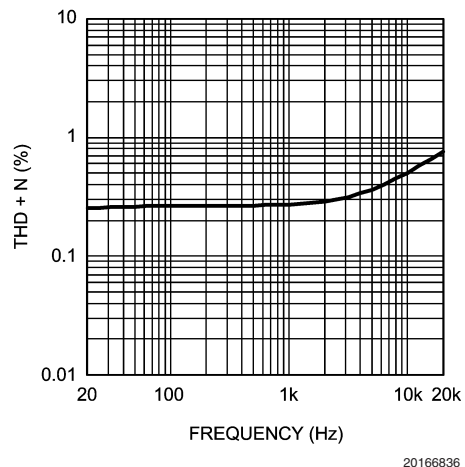
THD+N vs Frequency V_{DD} = 5V , R_L = 8\Omega , P_O = 500mW Mode 5
