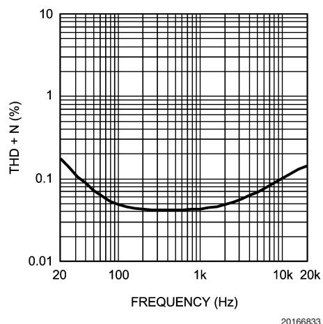
THD+N vs Frequency V_{DD} = 5V , R_L = 32\Omega , P_O = 30mW Mode 6, SE
