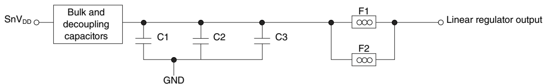
Figure 55. \text{SV}_{\text{DD}} power supply filter circuit
