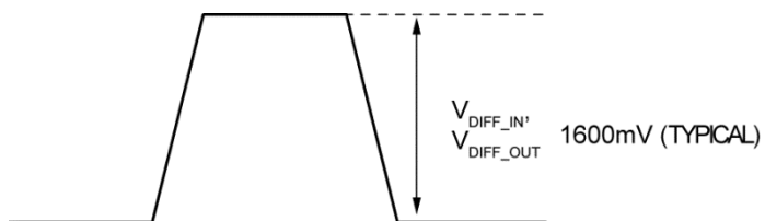
Figure 2. Differential Voltage Swing
