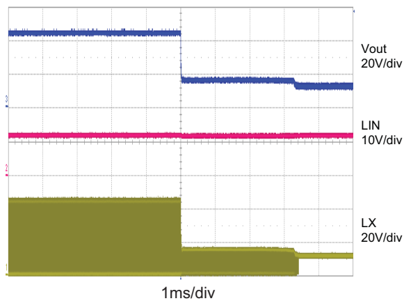
Output Short to GND (Soft-short)
