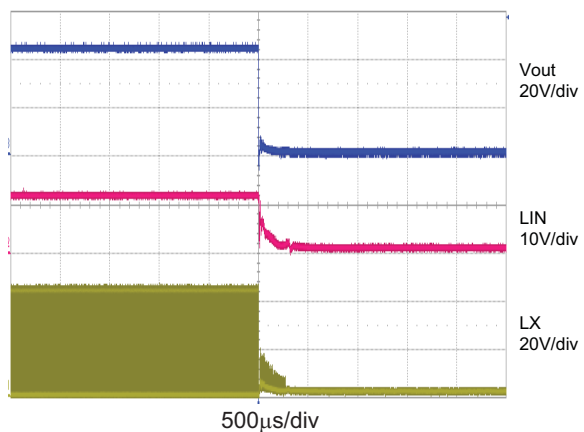
Output Short to GND (Hard-short)
