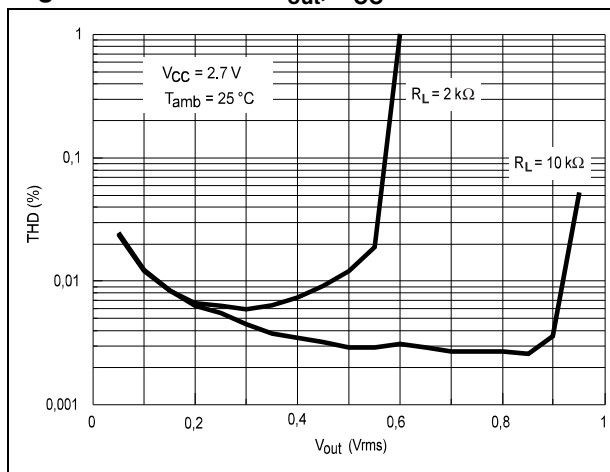
Figure 5. THD vs. V_{out} , V_{CC} = 2.7\text{ V}
