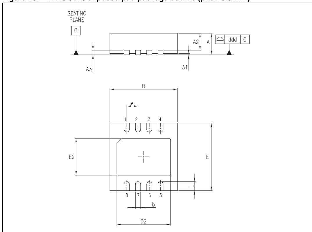
Figure 18. DFN8 3 x 3 exposed pad package outline (pitch 0.5 mm)
