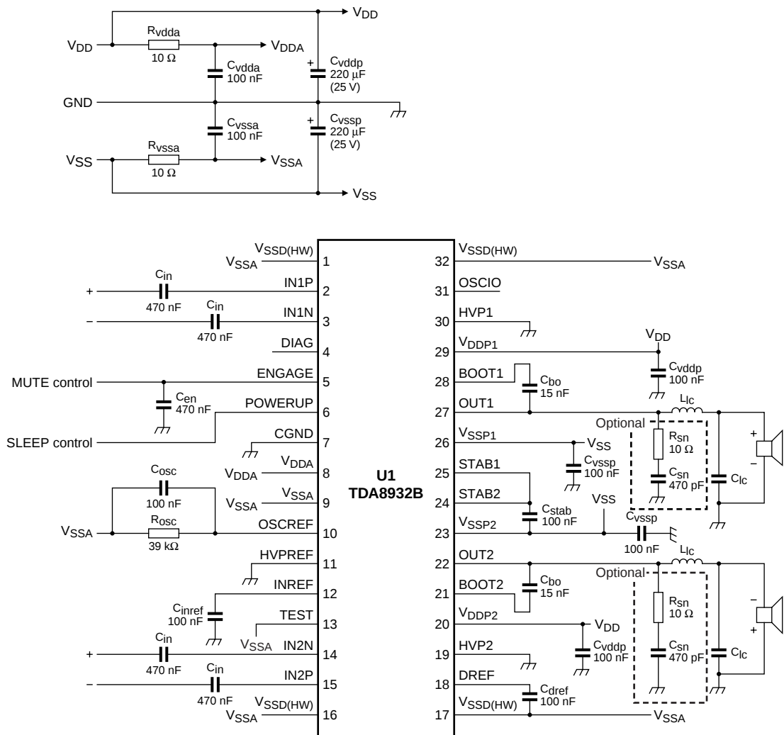
Fig 34. Typical simplified application diagram for 2 × SE (symmetrical supply)
