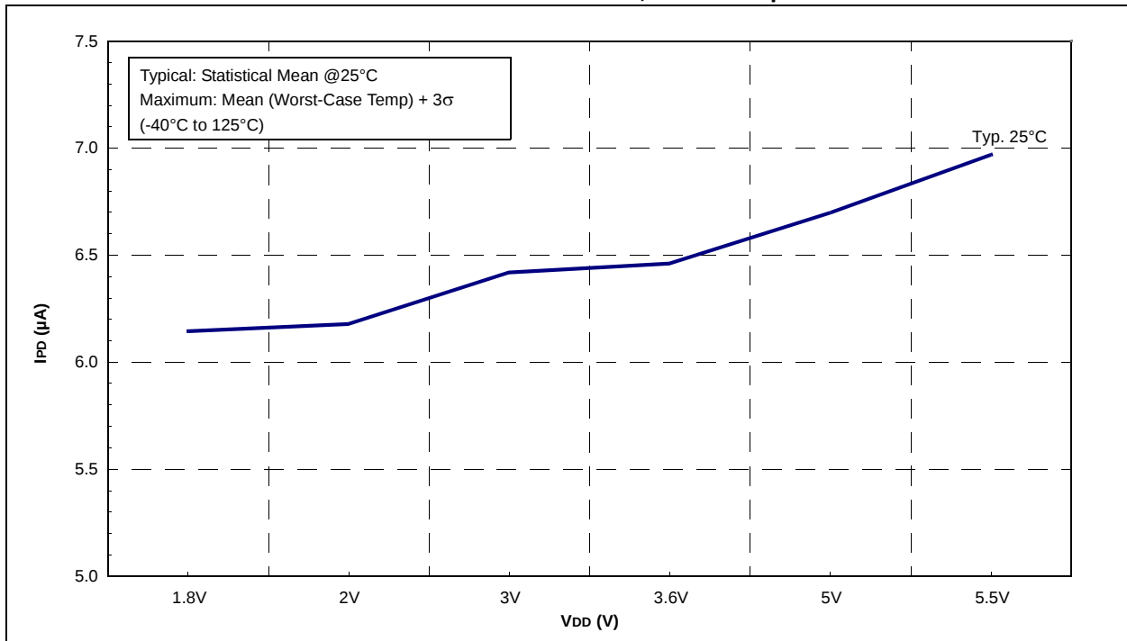
FIGURE 26-43: PIC16F707 TYPICAL ADC I PD vs. V DD , V CAP = 0.1μF
