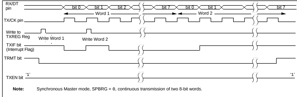
FIGURE 18-6: SYNCHRONOUS TRANSMISSION
