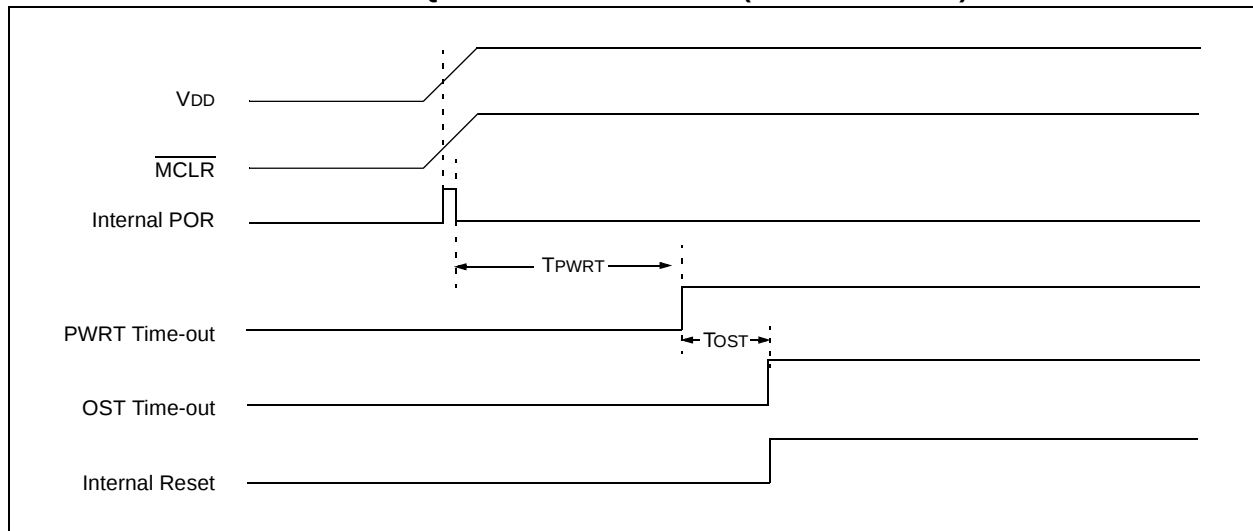
FIGURE 3-7: TIME-OUT SEQUENCE ON POWER-UP ( \overline{\text{MCLR}} WITH \text{VDD} ): CASE 3
