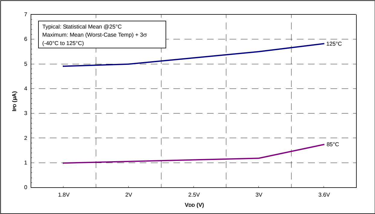
FIGURE 26-28: PIC16LF707 MAXIMUM BASE I PD vs. V DD
