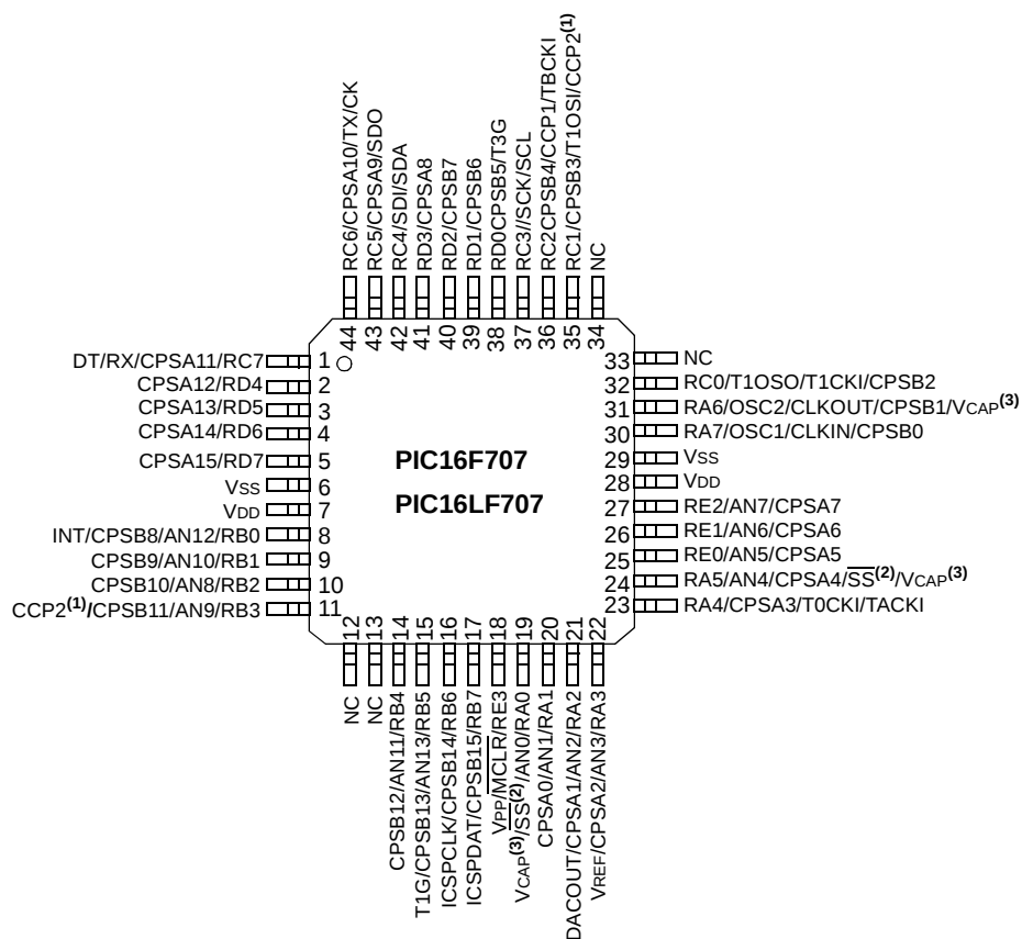
FIGURE 3: 44-PIN TQFP
