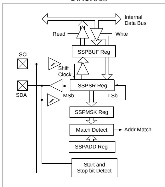
FIGURE 19-7: I 2 C MODE BLOCK DIAGRAM
