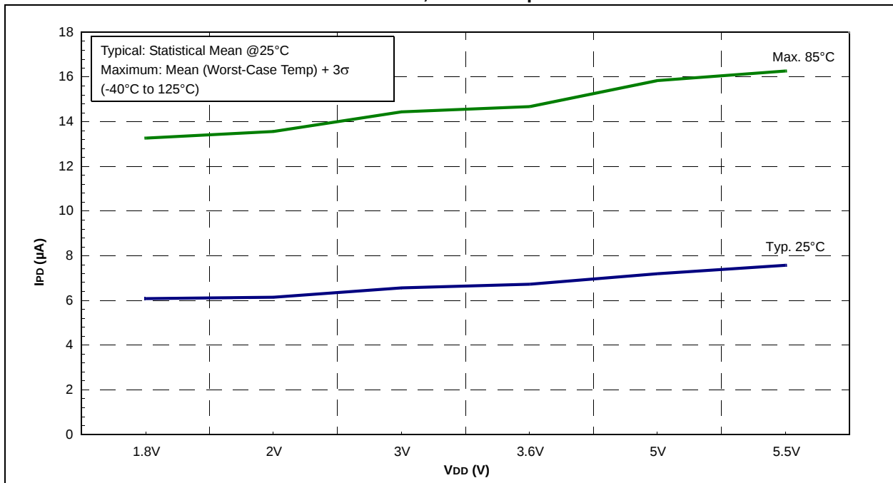
FIGURE 26-47: PIC16F707 WDT I_{PD} vs. V_{DD} , V_{CAP} = 0.1\mu F
