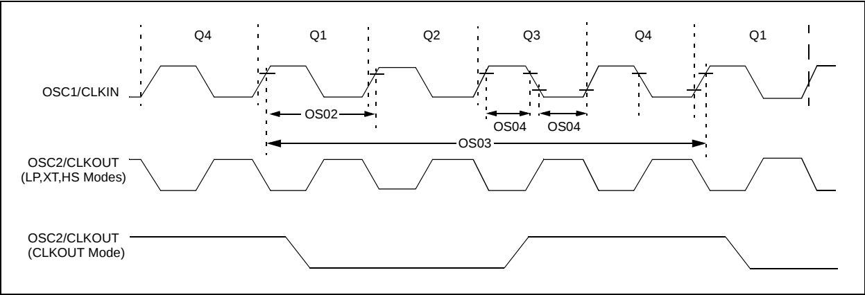
FIGURE 25-3: CLOCK TIMING
