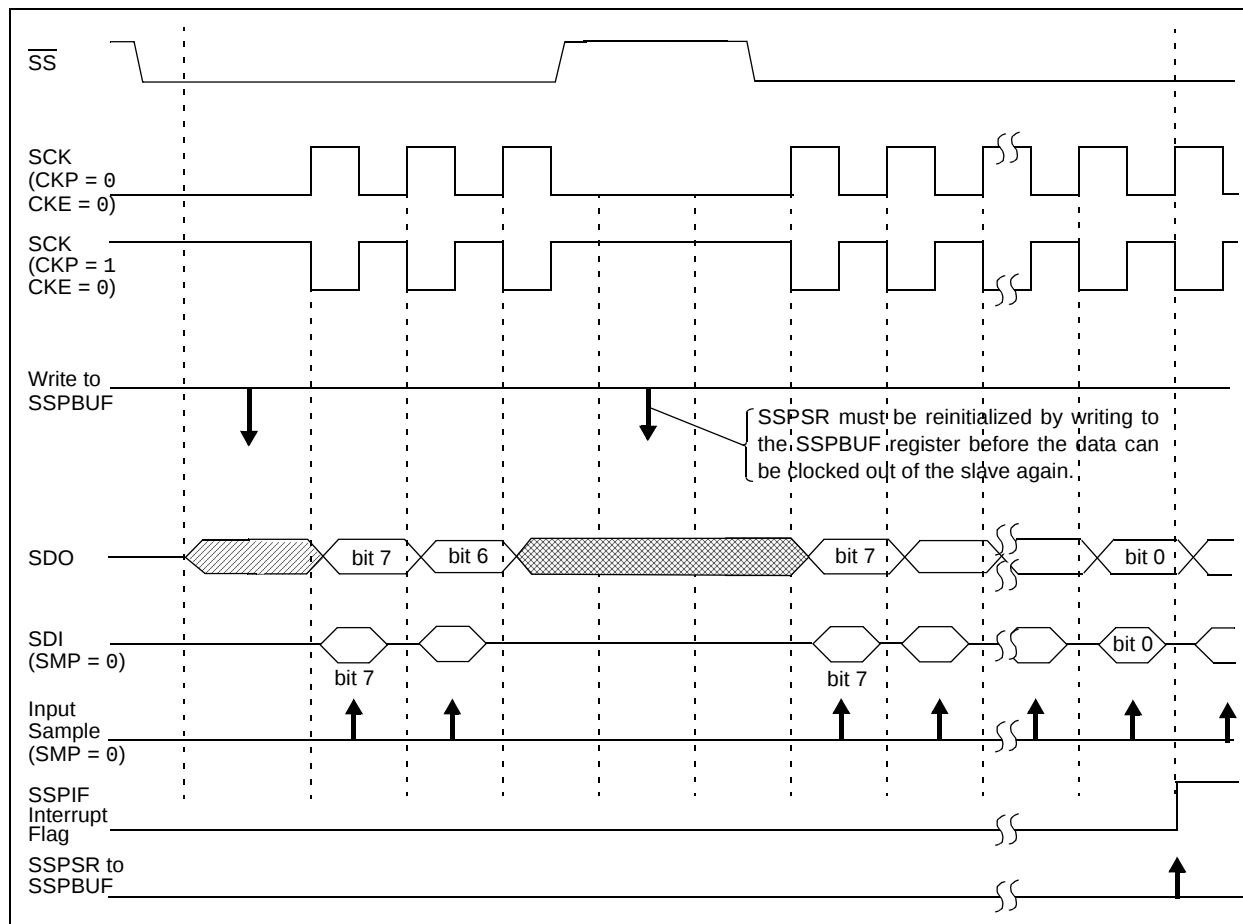
FIGURE 19-6: SLAVE SELECT SYNCHRONIZATION WAVEFORM
