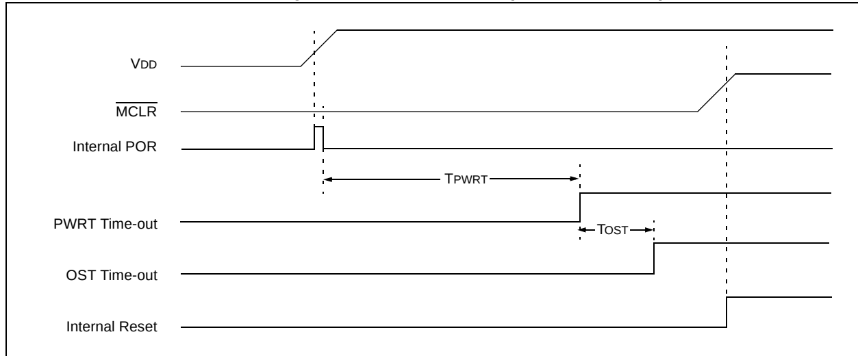
FIGURE 3-6: TIME-OUT SEQUENCE ON POWER-UP (DELAYED \overline{\text{MCLR}} ): CASE 2
