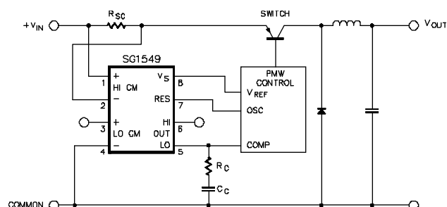
FIGURE 1 — HIGH LINE SENSING WITH THE SG1549 IN CONJUNCTION WITH AN SG1524 PWM CONTROL IC
