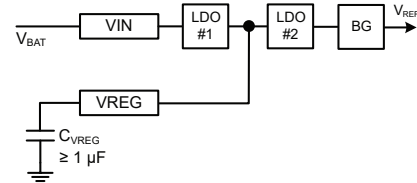
Figure 17: Internal LDOs and V_{REF} depend on C_{VREG}
