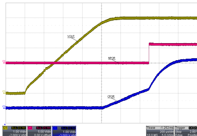
Figure 10: Operation of CPOR and NPOR
