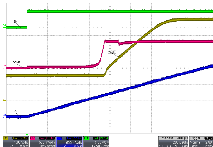
Figure 9: Startup with V OUT Pre-Biased to 1.5 V
