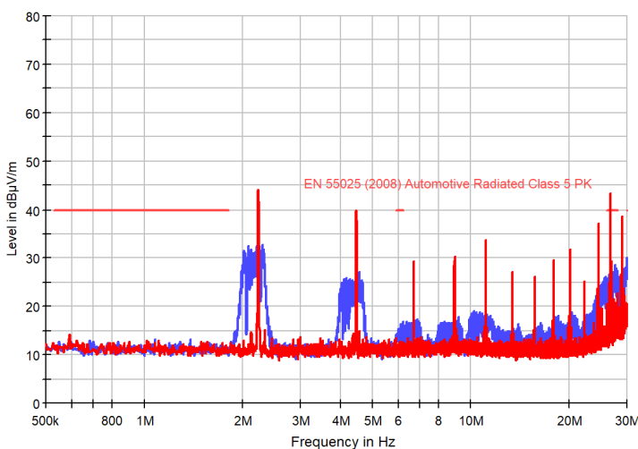
Figure 5: Comparison of Dithering (blue) to Non-Dithering (red) Radiated Emissions (Peak) in dBμV/m
