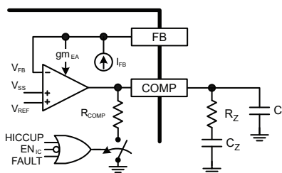
Figure 7: The A8660 Error Amplifier
