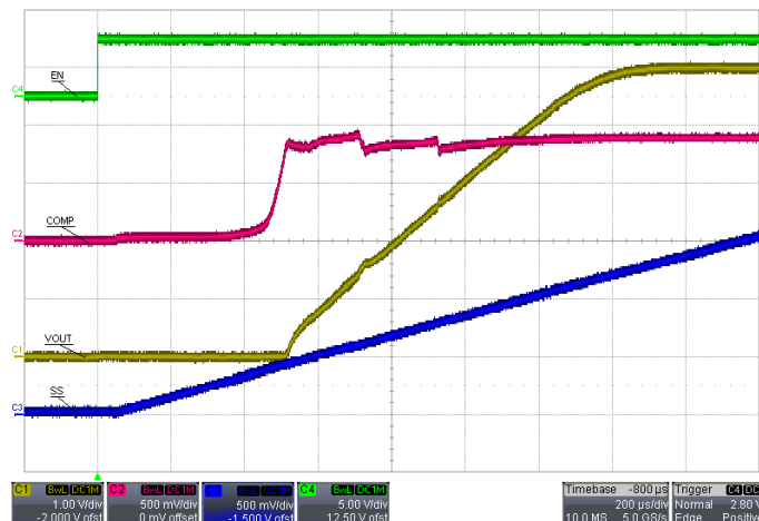
Figure 8: Soft-Start Operation
