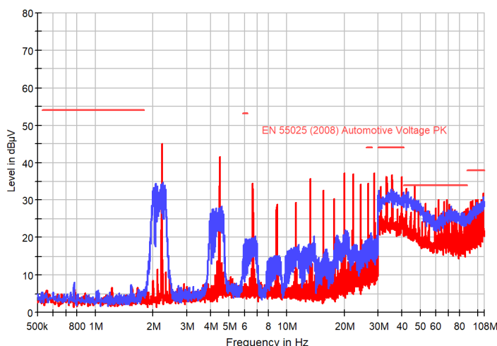
Figure 4: Comparison of Dithering (blue) to Non-Dithering (red) Conducted Emissions (Peak) in dBμV
