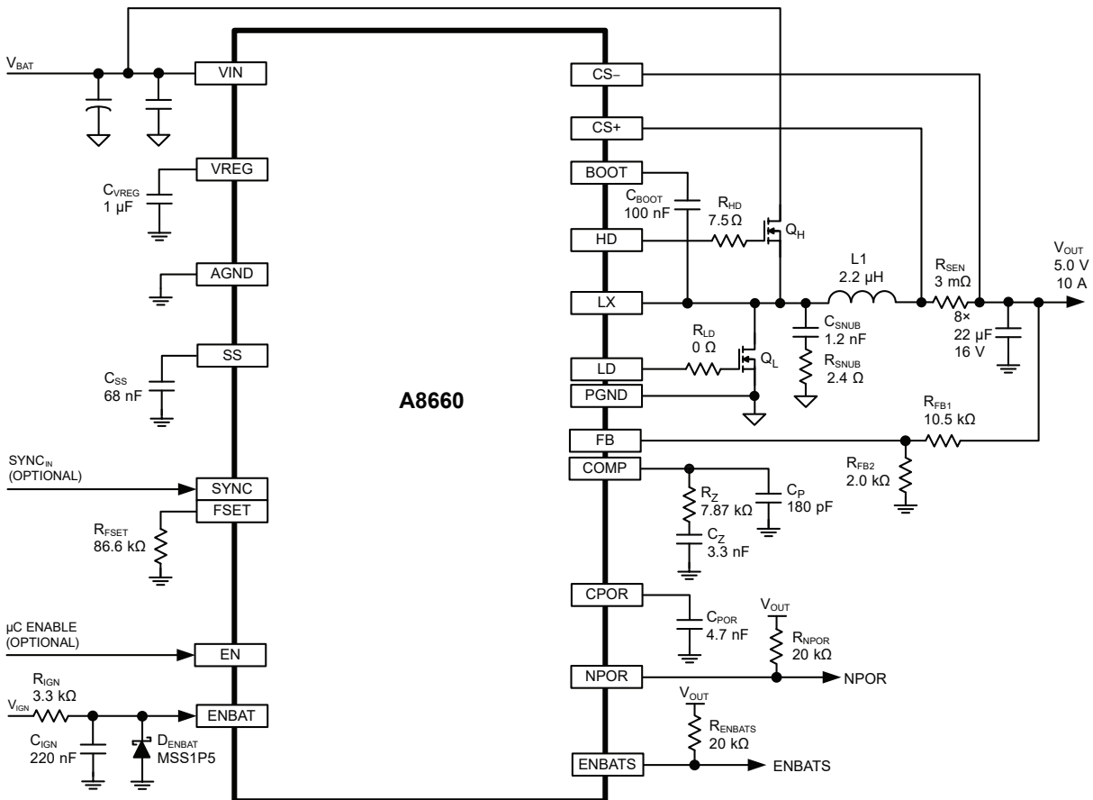
Figure 3: Low Frequency Design Example: 12 V_{IN} , 5 V_{OUT} , 10 A at 410 kHz
