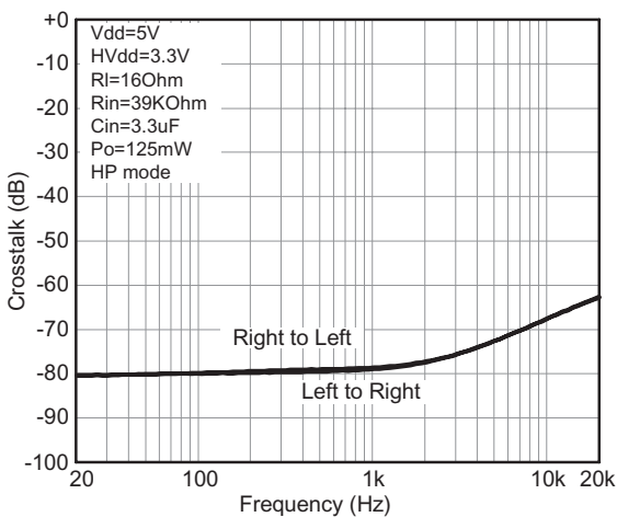
Figure 24. Crosstalk vs. Frequency
