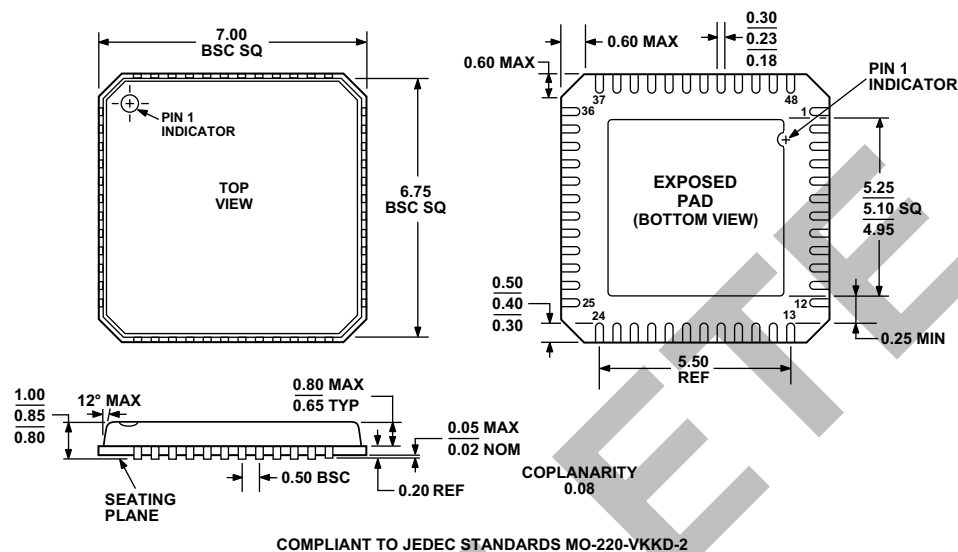
Figure 3. 48-Lead, Lead Frame Chip Scale Package [LFCSP_VQ] 7 mm x 7 mm Body, Very Thin Quad (CP-48-1)
