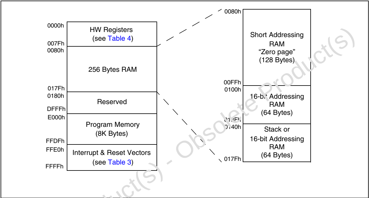
Figure 6. Memory Map
