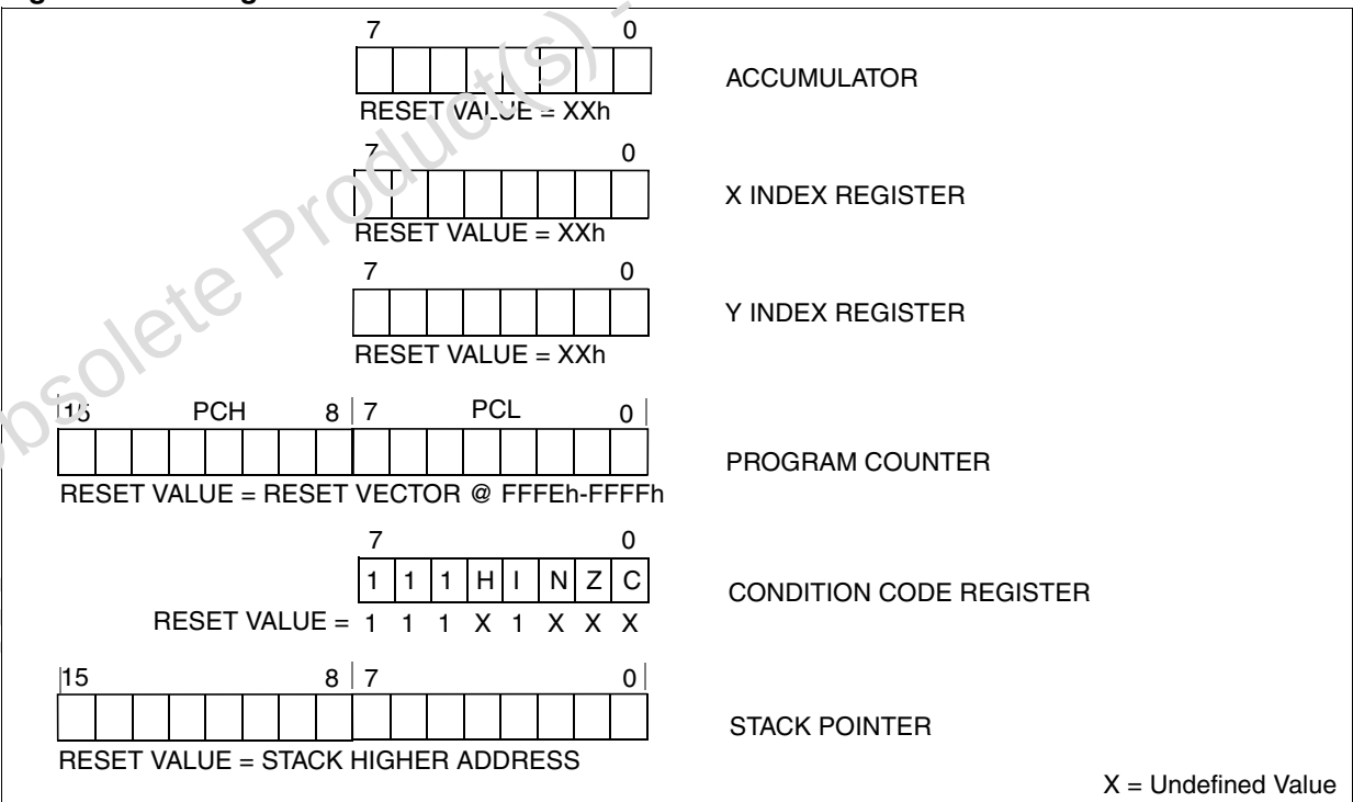
Figure 7. CPU Registers
