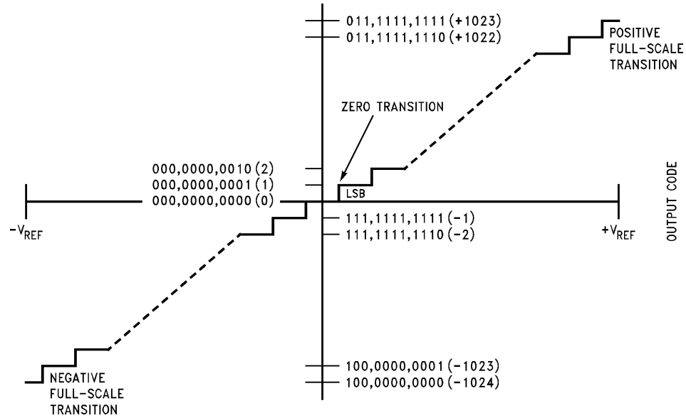
FIGURE 1. Transfer Characteristic
