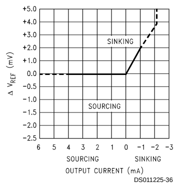
Load Regulation
