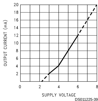
Available Output Current vs Supply Voltage
