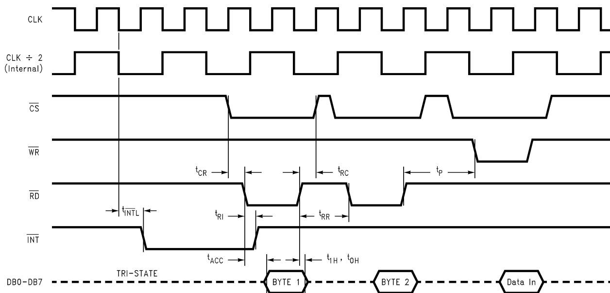
DIAGRAM 3. Reading the Conversion Result
