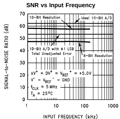
FIGURE 7. ADC10154/ADC10158 Signal-to-Noise Ratio vs Input Frequency
