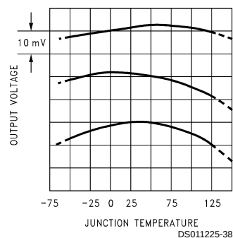
Output Drift vs Temperature (3 Typical Parts)
