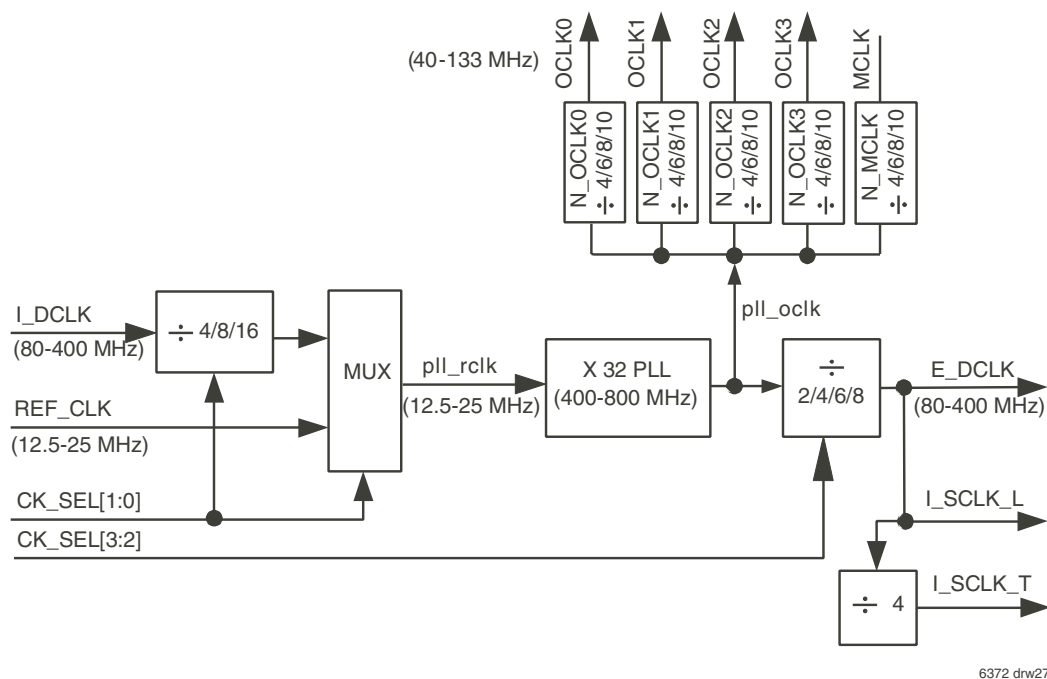
Figure 29. Clock generator
