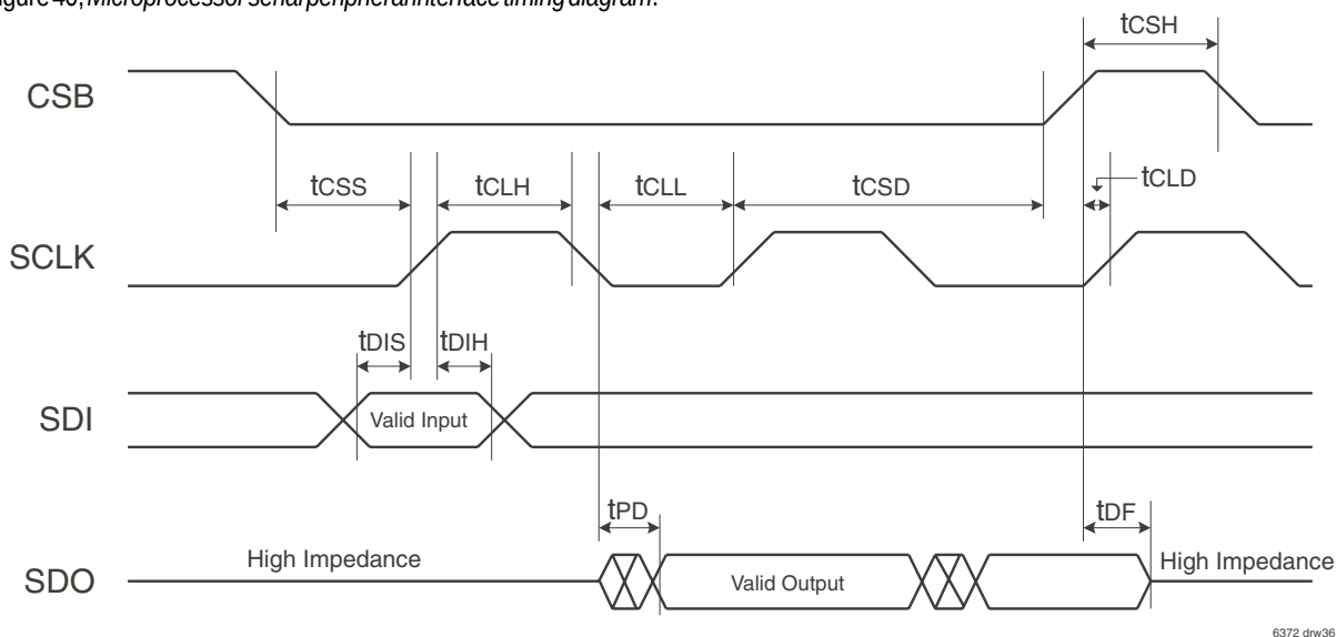
Figure 40. Microprocessor serial peripheral interface timing diagram
