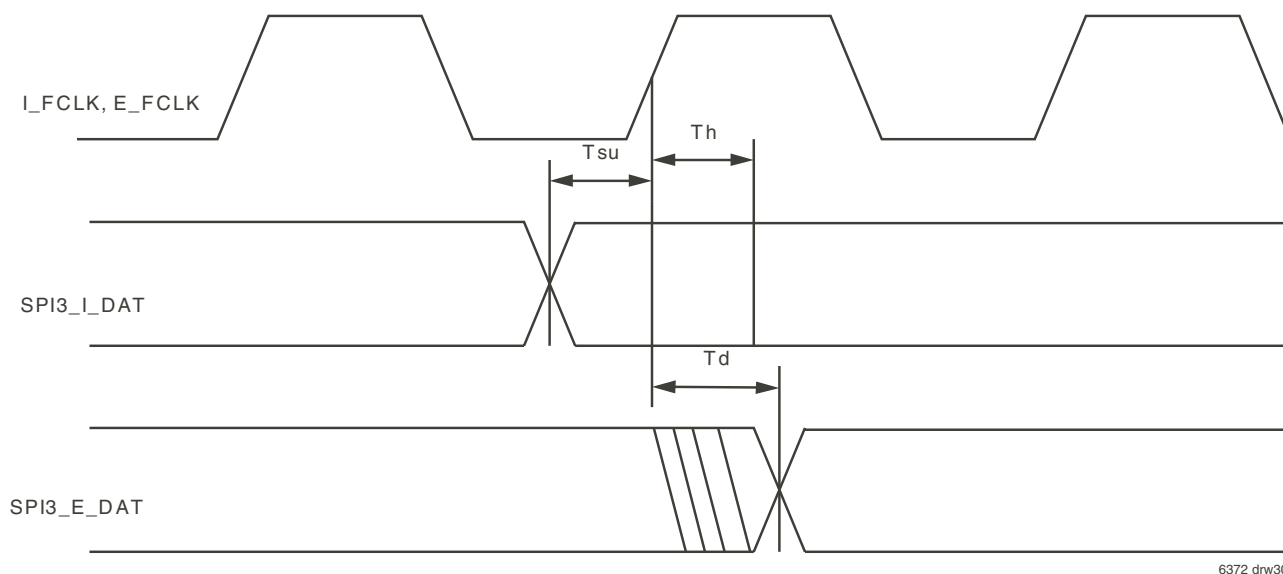
Figure 34. SPI-3 I/O timing diagram
