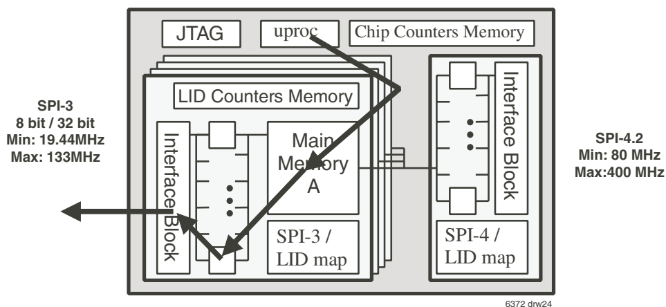
Figure 24. Microprocessor interface to SPI-3 egress detailed datapath diagram
