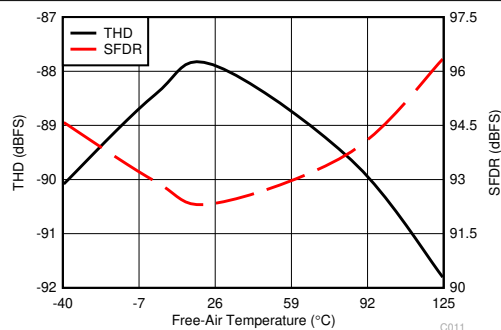
Figure 6-16. Distortion Performance vs Temperature
