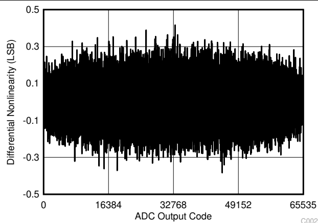
Figure 6-3. Typical DNL
