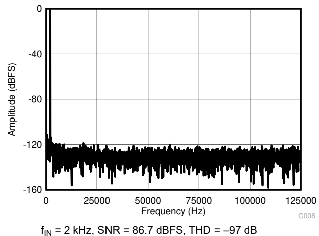
Figure 6-14. Typical FFT
