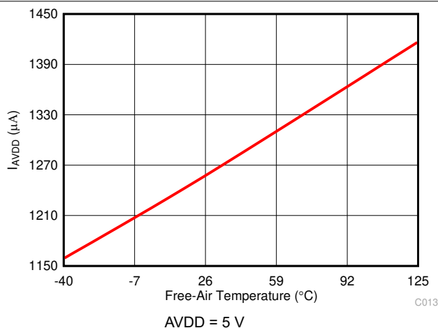
Figure 6-19. Analog Supply Current vs Temperature
