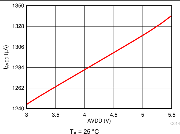
Figure 6-20. Analog Supply Current vs AVDD
