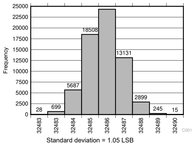
Figure 6-13. DC Input Histogram
