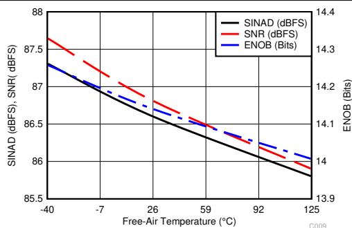
Figure 6-15. Noise Performance vs Temperature
