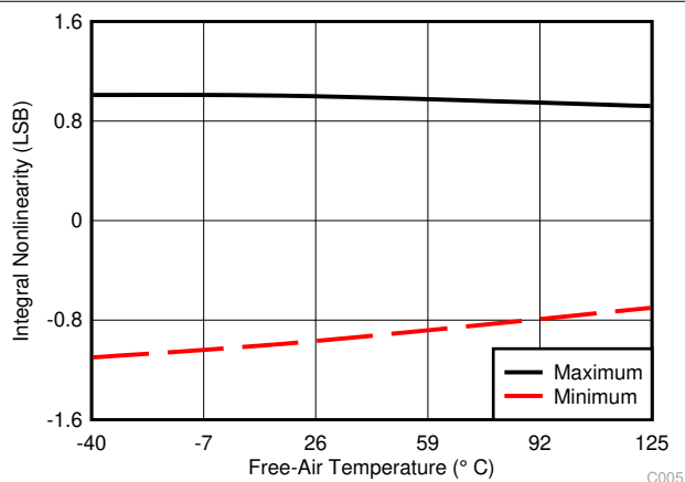
Figure 6-4. Typical INL
