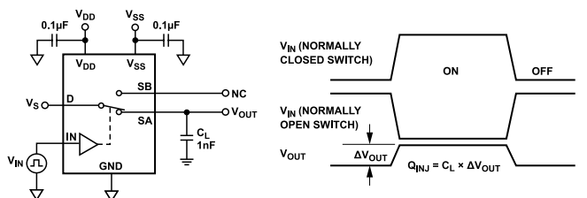
Figure 24. Charge Injection
