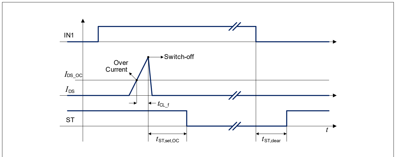
Figure 10 Overcurrent detection
