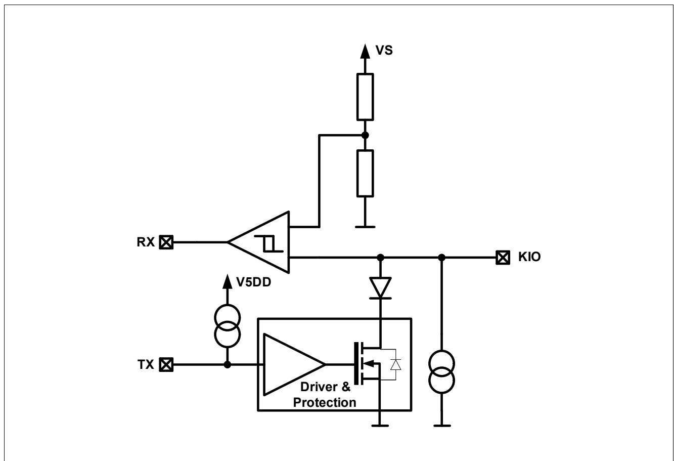
Figure 11 K-line block diagram
