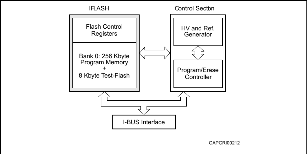
Figure 5. Flash structure
