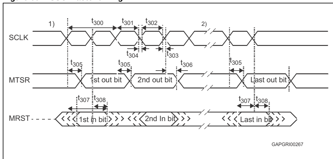
Figure 60. SSC master timing
