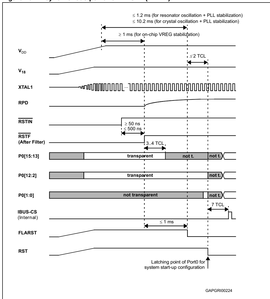
Figure 16. Asynchronous power-on RESET ( \overline{EA} = 1 )
