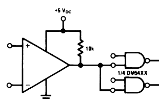
Driving TTL
