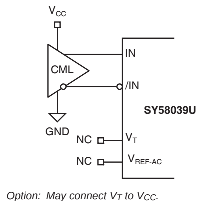
Figure 3c. CML Interface (DC-Coupled)
