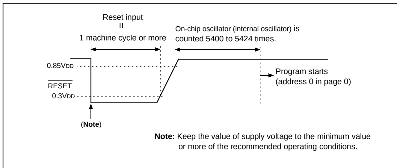
Fig. 38 \overline{\text{RESET}} pin input waveform and reset operation
