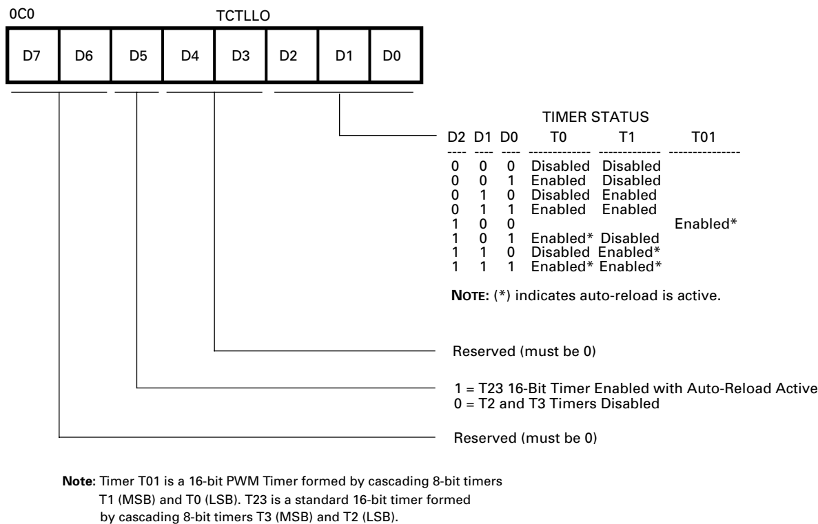
Figure 22. TCTLLO Register
