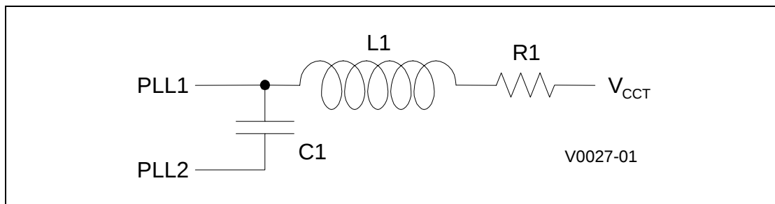
Figure 2. PLL RLC Filter
