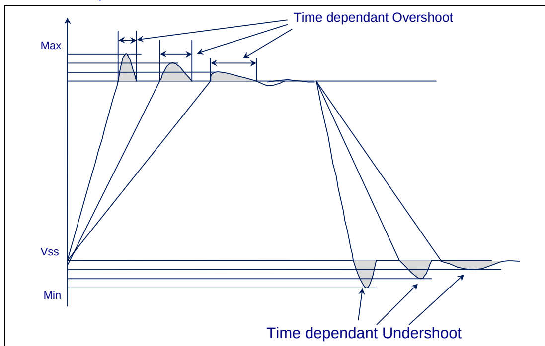
Figure 21. Maximum Acceptable Overshoot/Undershoot Waveform
