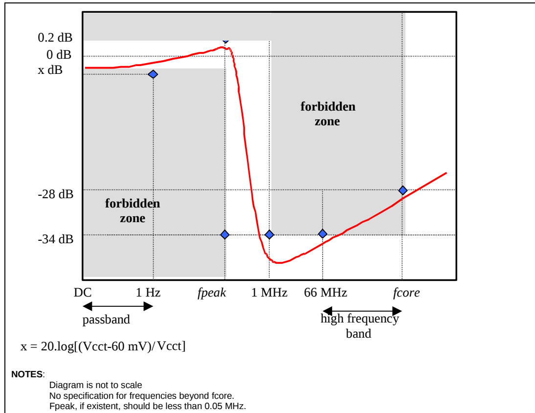
Figure 29. PLL Filter Specifications
