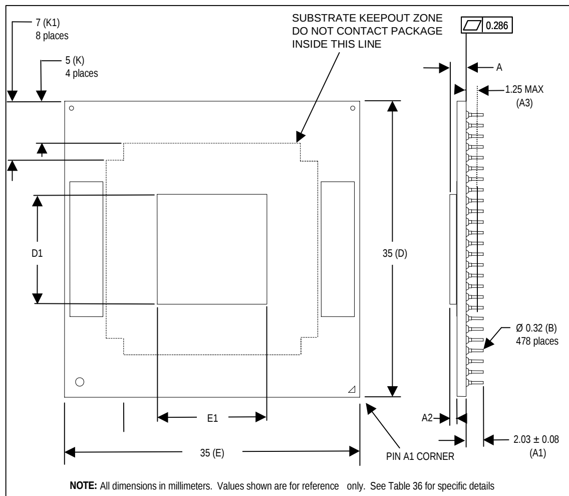
Figure 23. Socketable Micro-FCPGA Package - Top and Side View
