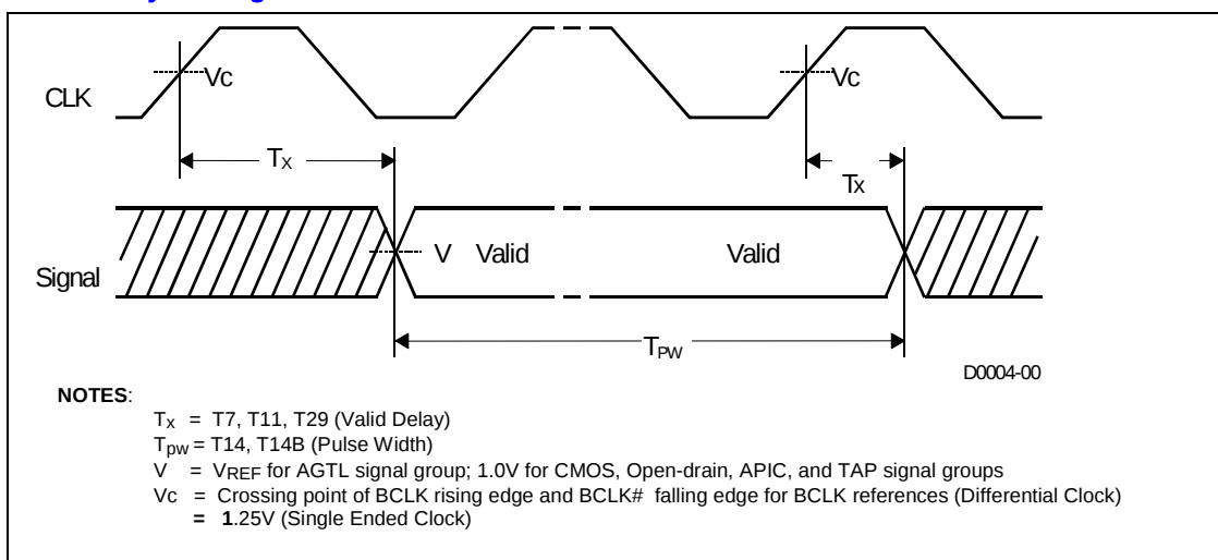
Figure 9. Valid Delay Timings
