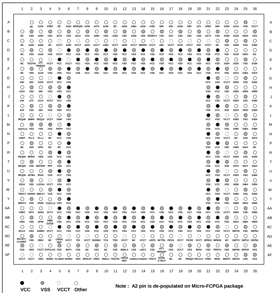
Figure 28. Pin/Ball Map - Top View
