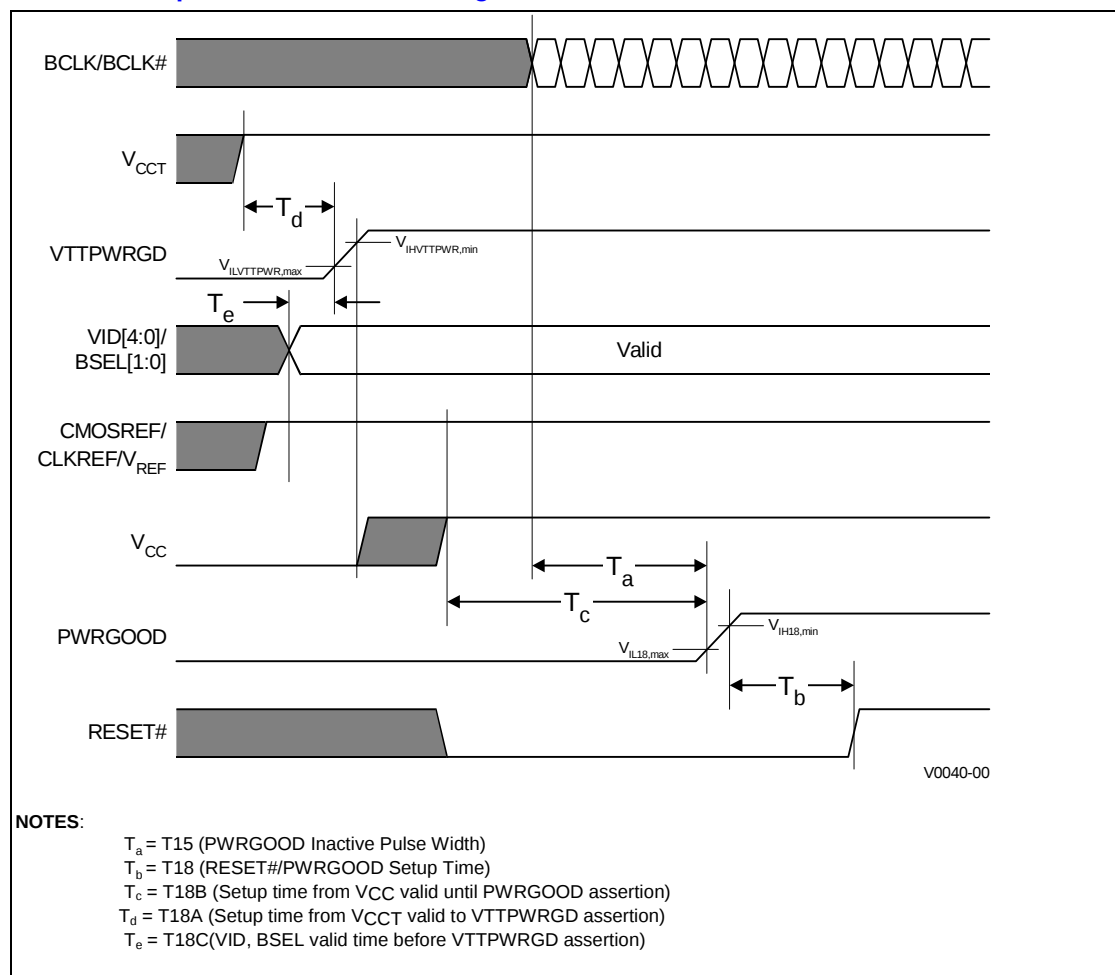
Figure 12. Power-on Sequence and Reset Timings
