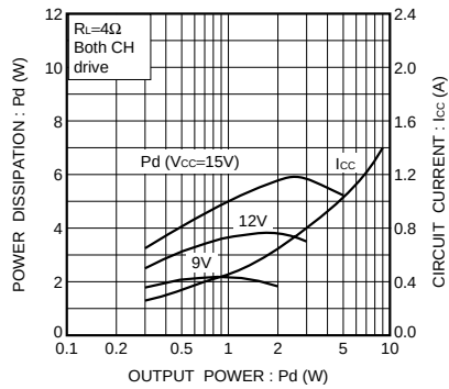
Fig.31 Power dissipation and current vs. power supply voltage (RL=4Ω)
