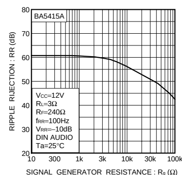
Fig.27 Ripple rejection vs. signal source resistance (BA5415A)
