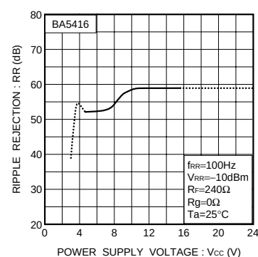
Fig.24 Ripple rejection vs. power supply voltage (BA5416)
