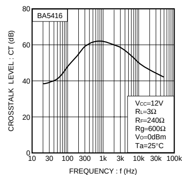
Fig.21 Crosstalk vs. frequency (BA5416)
