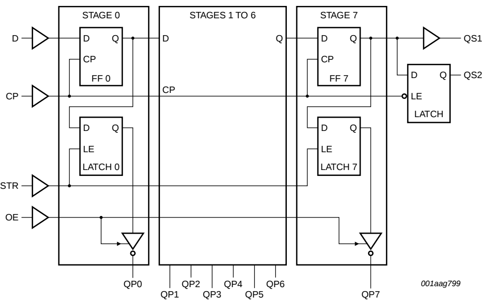
Fig 4. Logic diagram
