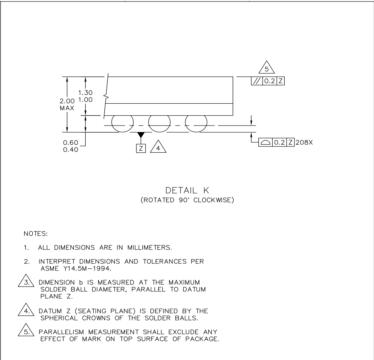
TITLE: 208 I/O MAP BGA, 17 X 17 PKG, 1-MM PITCH CASE NUMBER: 1159A-01 STANDARD: JEDEC MO-151 AAF-1 PACKAGE CODE: 5253 SHEET: 2
