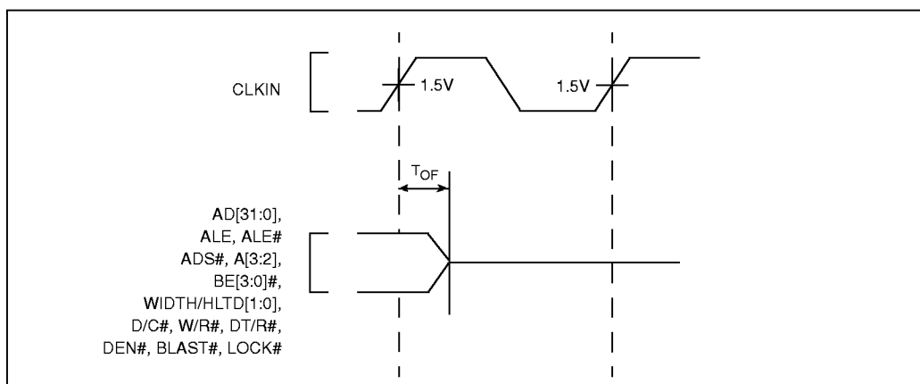
Figure 26. T_{IS1} and T_{IH1} Input Setup and Hold Waveform
