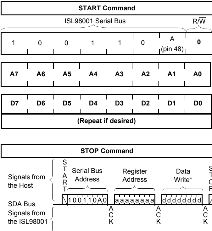
FIGURE 12. CONFIGURATION REGISTER WRITE
