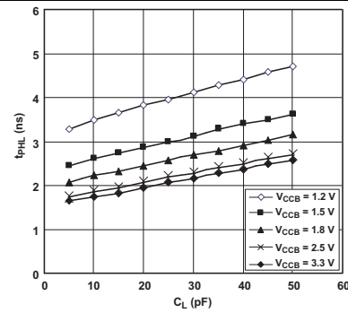
Figure 2. Typical A-to-B Propagation Delay, High to Low
