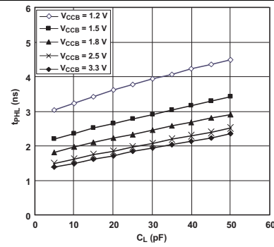
Figure 4. Typical A-to-B Propagation Delay, High to Low
