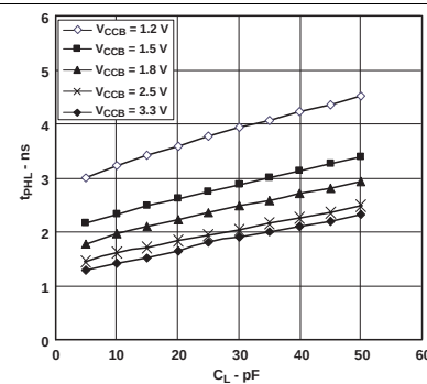
Figure 6. Typical A-to-B Propagation Delay, High to Low
