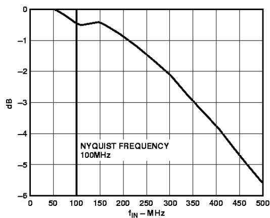
Figure 24. Frequency Response: f_S = 200 MSPS
