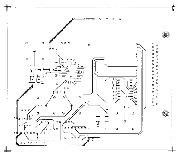
Figure 41. Conductors—Top View
