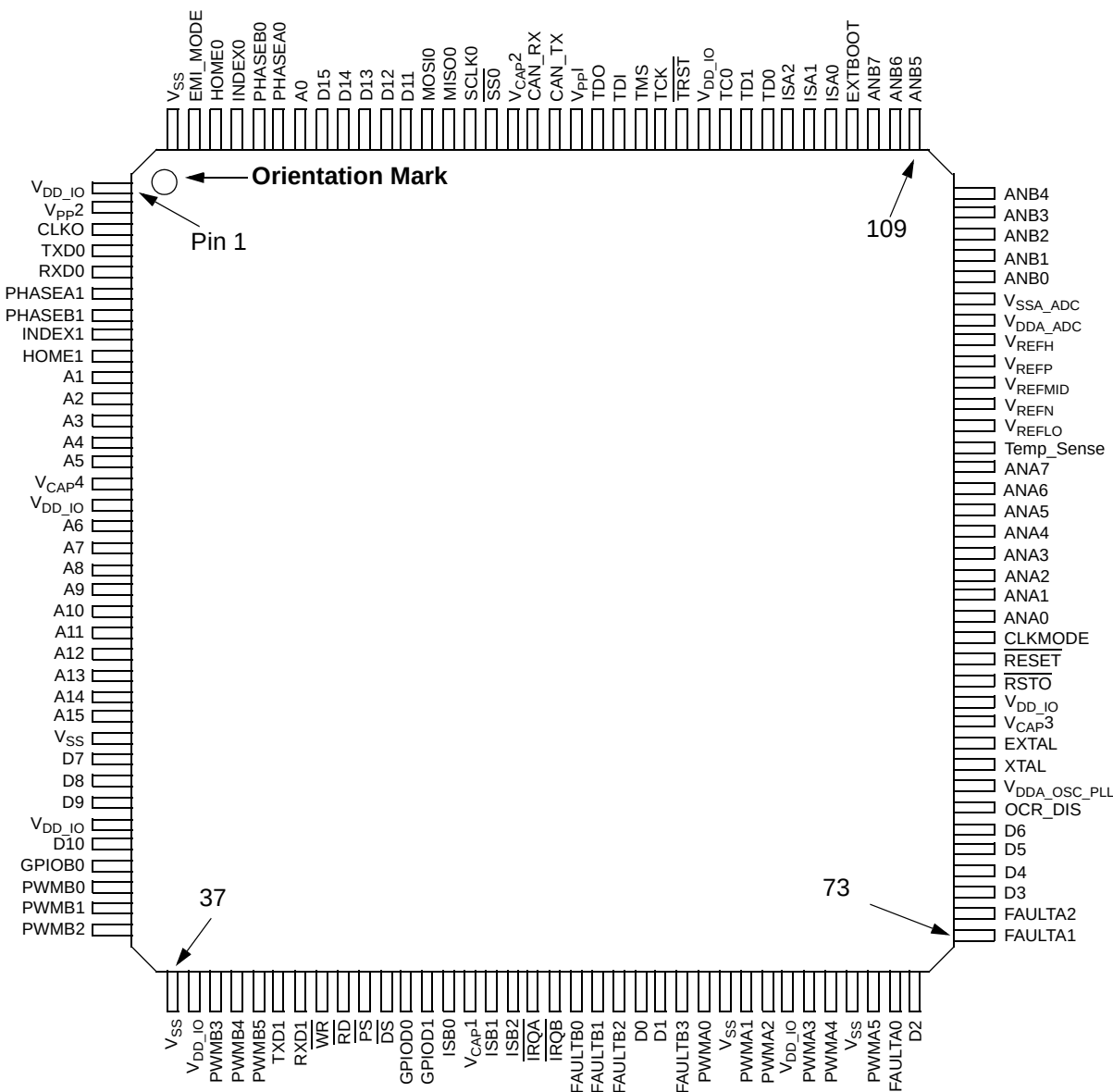
Figure 11-1 Top View, 56F8346 144-Pin LQFP Package
