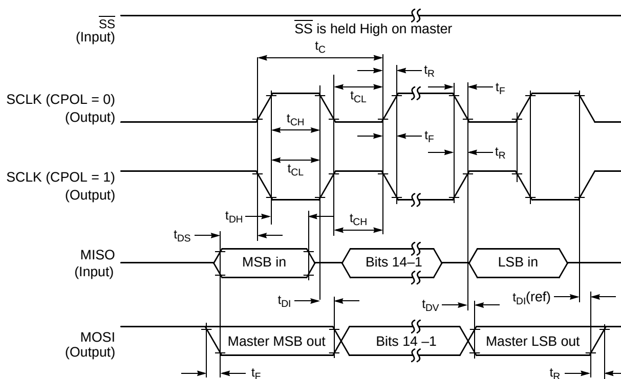
Figure 10-10 SPI Master Timing (CPHA = 0)
