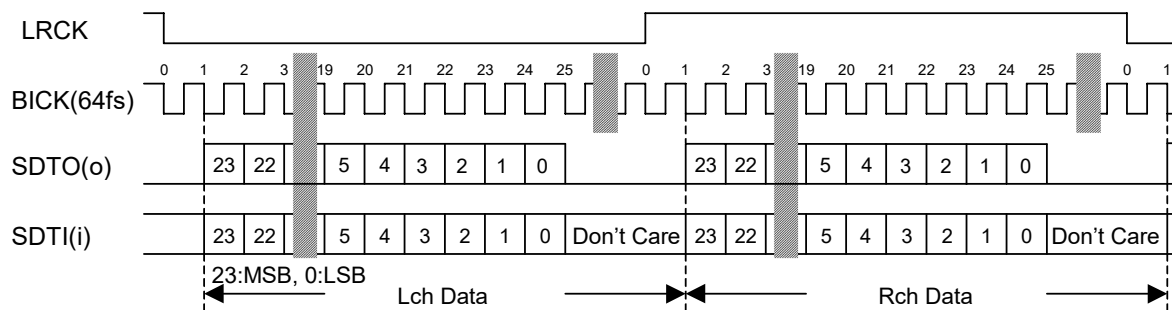
Figure 4. Mode 3 Timing
