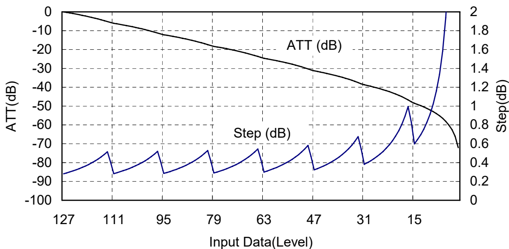
Figure 9. ATT characteristics
