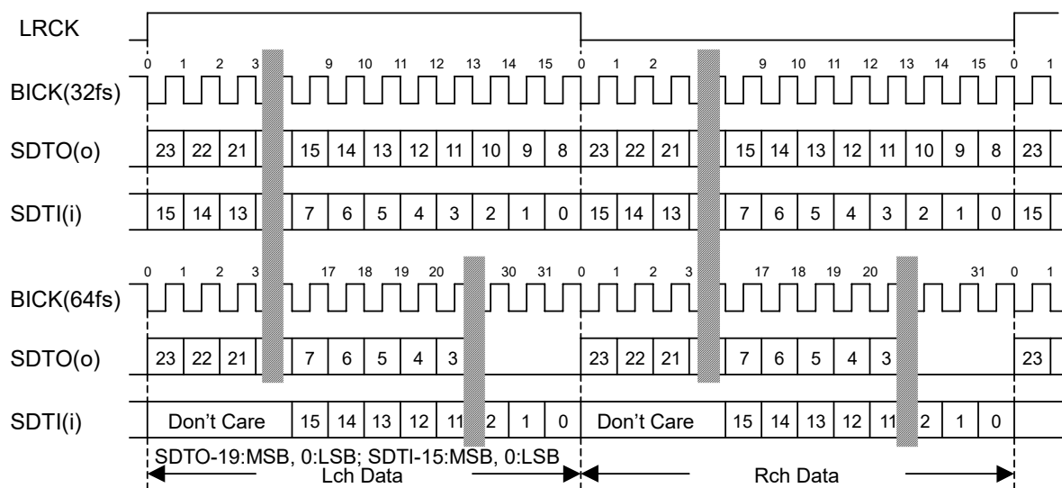
Figure 1. Mode 0 Timing
