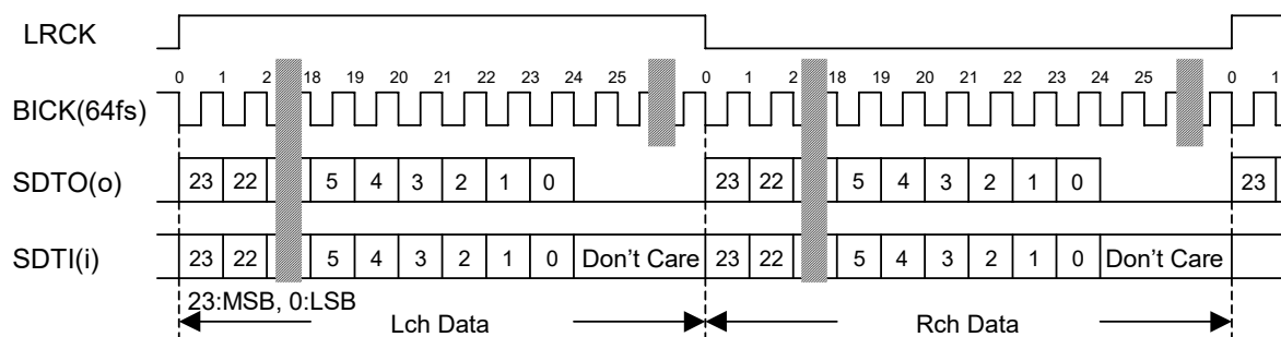
Figure 3. Mode 2 Timing
