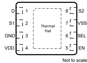
Figure 5-2. RQX Package, 8-Pin WSON (Top View)
