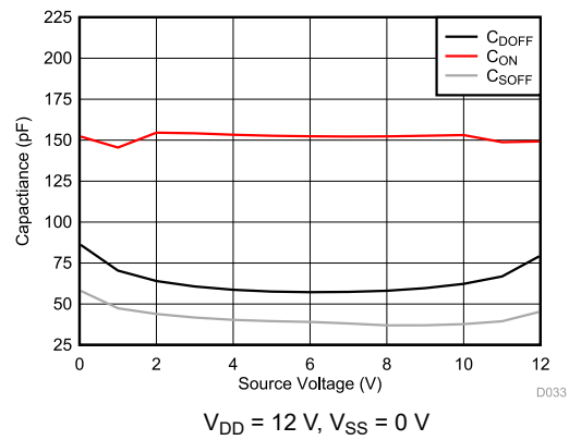
Figure 6-31. Capacitance vs Source Voltage or Drain Voltage
