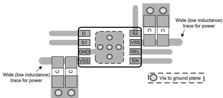
Figure 11-3. TMUX7219RQX Layout Example
