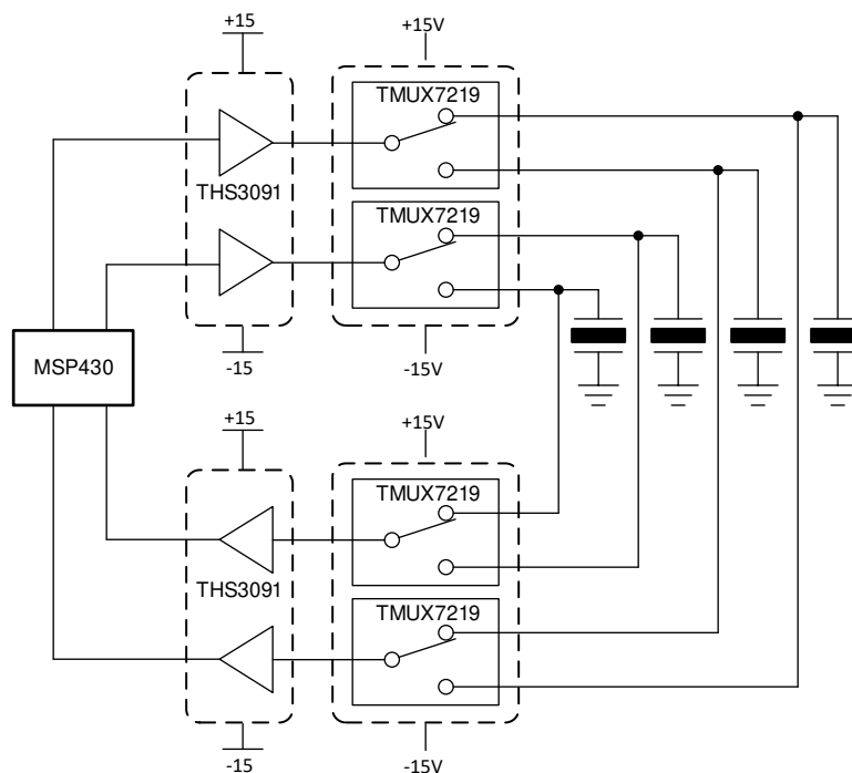
Figure 9-3. Ultrasonic Sensing Gas Meter System
