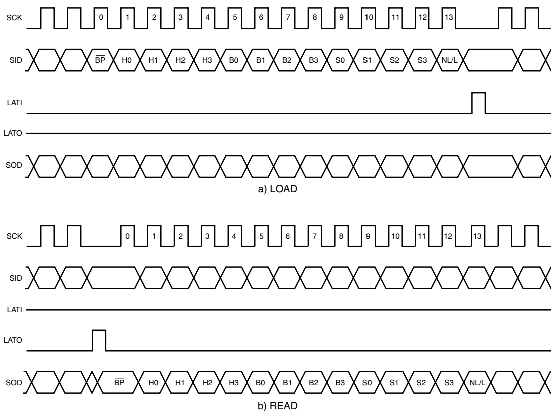
Figure 6. Serial Timing
