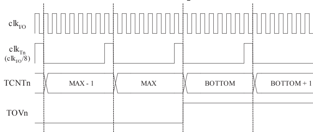
Figure 19-4 Timer/Counter Timing Diagram, with Prescaler ( f_{\text{clk\_I/O}}/8 )
