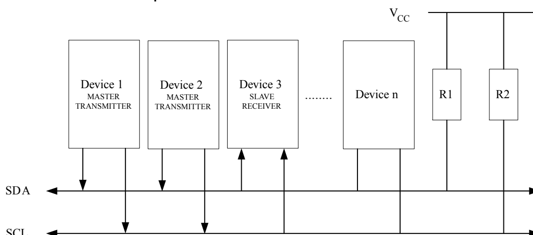
Figure 25-20 An Arbitration Example
