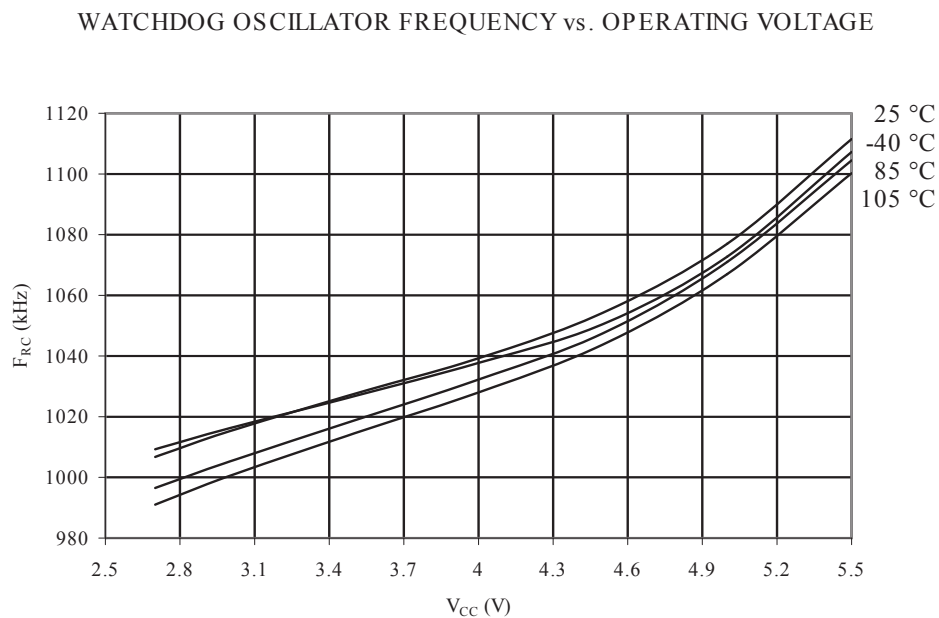
Figure 33-35 Watchdog Oscillator Frequency vs. V_{CC}
