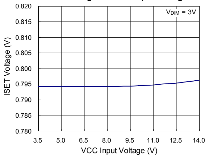
ISET Voltage vs. VCC Input Voltage
