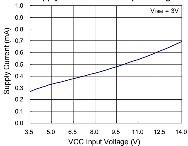
Supply Current vs. VCC Input Voltage
