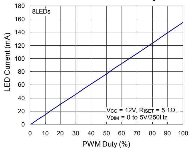
LED Current vs. PWM Duty
