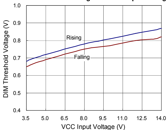
DIM Threshold Voltage vs. VCC Input Voltage
