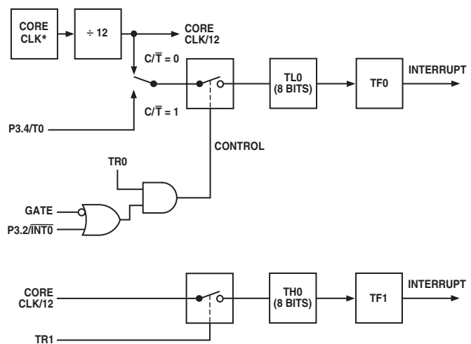
Figure 51. Timer/Counter 0, Mode 3
