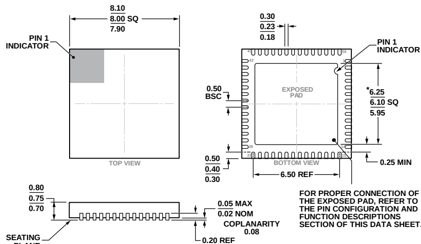
*COMPLIANT TO JEDEC STANDARDS MO-220-WLLD-2 WITH EXCEPTION TO EXPOSED PAD DIMENSION. Figure 81. 56-Lead Lead Frame Chip Scale Package [LFCSP] 8 x 8 mm Body and 0.75 mm Package Height (CP-56-11) Dimensions shown in millimeters
