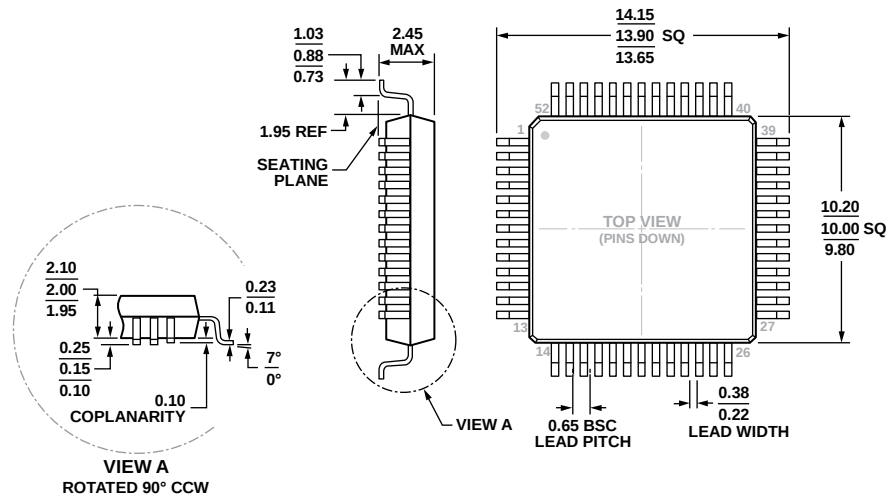
Figure 80. 52-Lead Metric Quad Flat Package [MQFP] (S-52-2) Dimensions shown in millimeters
