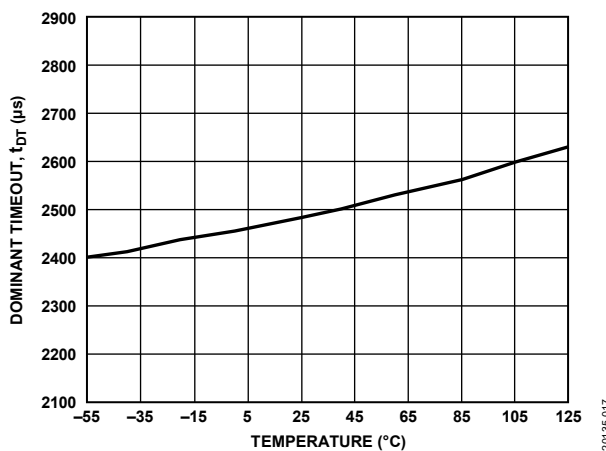
Figure 16. Dominant Timeout ( t_{DT} ) vs. Temperature
