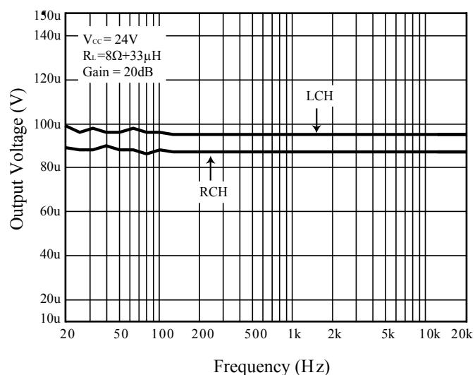
Figure 20 Noise
