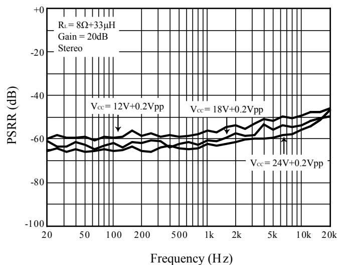
Figure 18 PSRR
