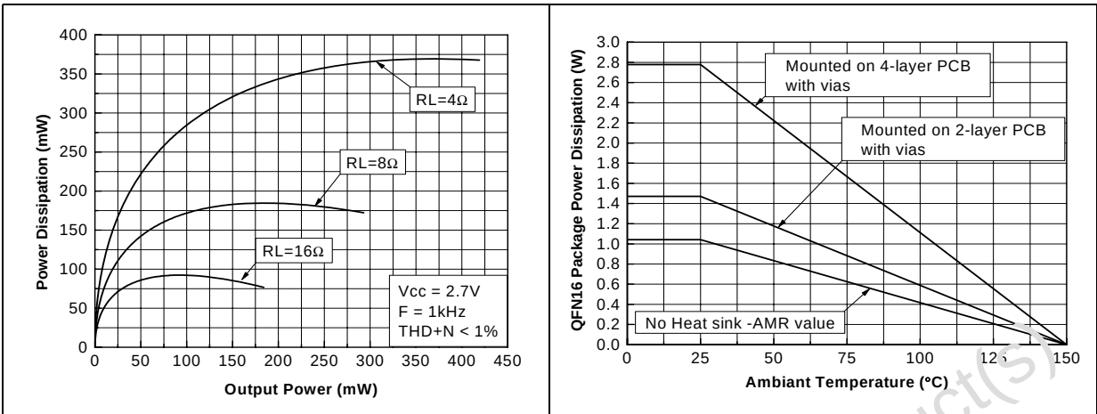
Figure 62. Power dissipation vs. output power Figure 63. Power derating curves
