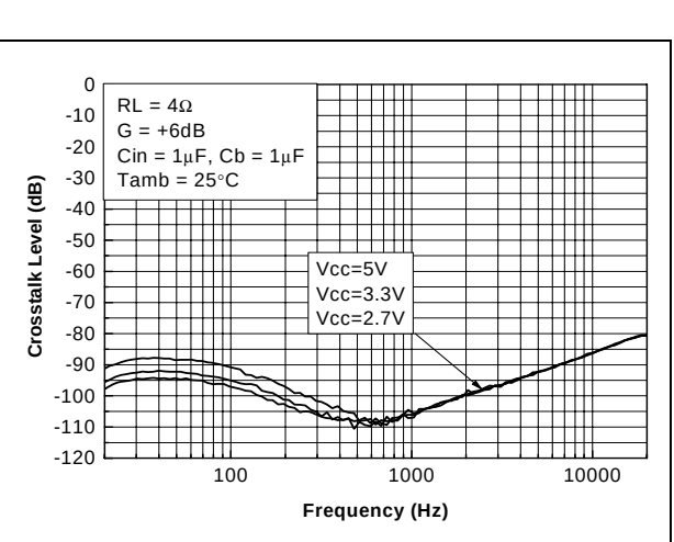
Figure 37. Crosstalk vs. frequency
