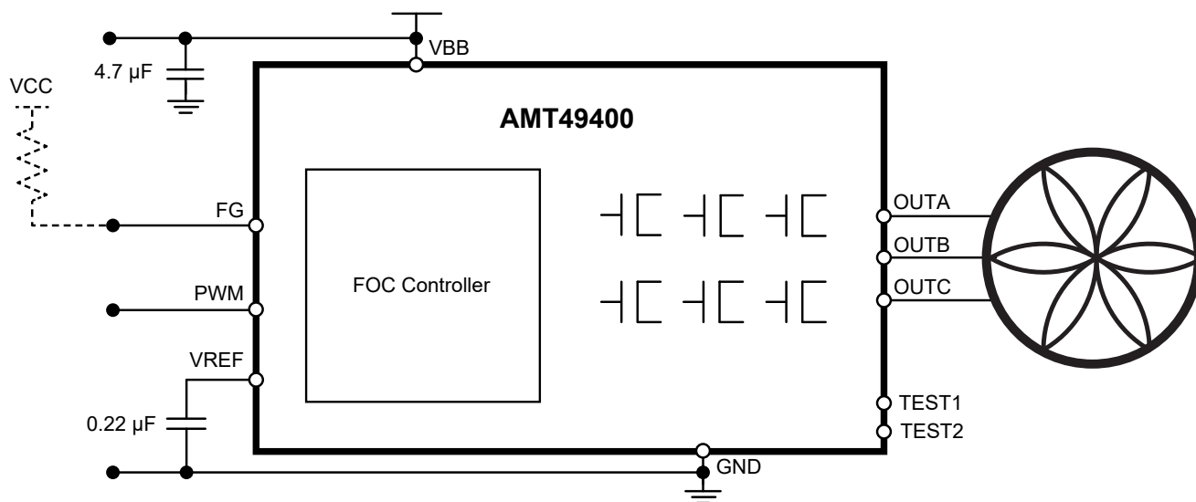
Figure 1: Typical Application
