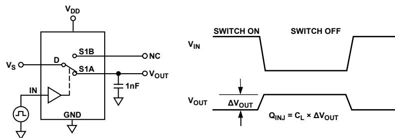
Figure 26. Charge Injection
