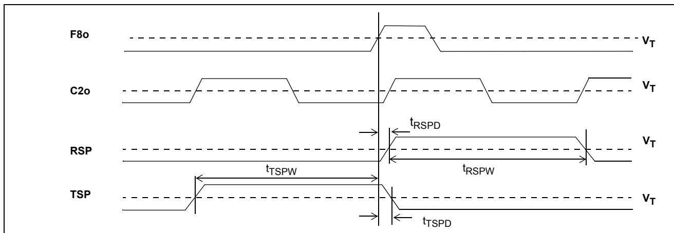
Figure 15 - Output Timing 2
