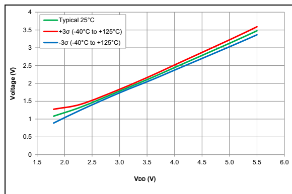
FIGURE 36-101: Schmitt Trigger High Values
