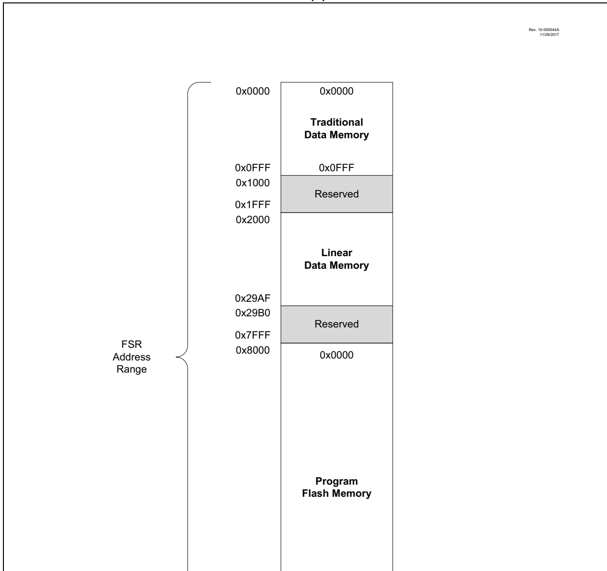
FIGURE 4-8: INDIRECT ADDRESSING PIC16(L)F18326/18346
