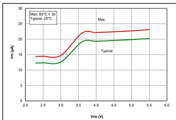
FIGURE 36-14: I_{PD} Base, 01 (PIC16F18326/46 only)
