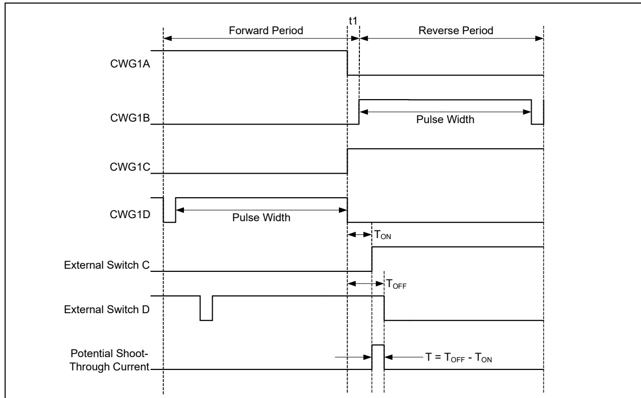
FIGURE 20-7: EXAMPLE OF PWM DIRECTION CHANGE AT NEAR 100% DUTY CYCLE
