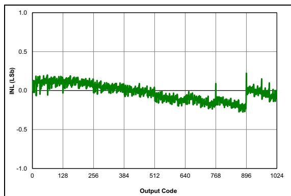
FIGURE 36-54: ADC 10-Bit Mode, Single-Ended INL, V_{DD} = 3.0V , V_{REF} = 3.0V , T_{AD} = 1\text{ }\mu S , 25C (All devices)
