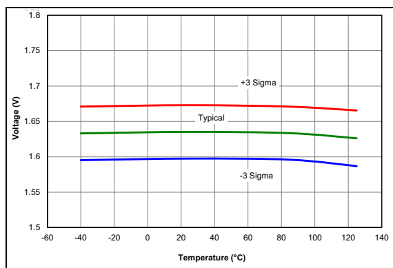
FIGURE 36-110: POR Rearm Voltage, Normal Power Mode
