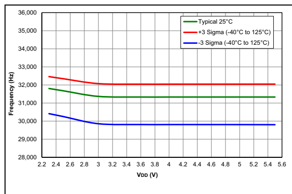
FIGURE 36-29: LFINTOSC Frequency (PIC16F18326/46 only)
