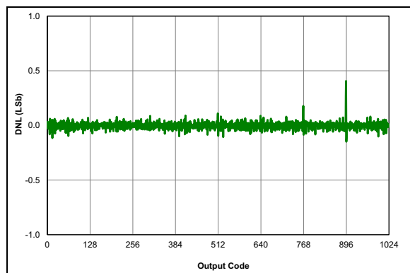
FIGURE 36-53: ADC 10-Bit Mode, Single-Ended DNL, V_{DD} = 3.0V , V_{REF} = 3.0V , T_{AD} = 8\text{ }\mu S , 25C (All devices)
