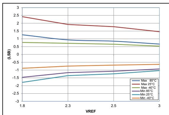
FIGURE 36-62: ADC 10-Bit Mode, Single-Ended Offset Error, V_{DD} = 3.0V , T_{AD} = 1\text{ }\mu s (All devices)
