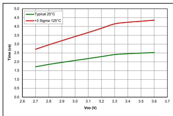
FIGURE 36-49: BOR Response Time (PIC16LF18326/46 only)
