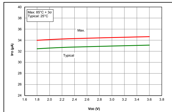
FIGURE 36-12: I_{PD} , Comparator (PIC16LF18326/46 only)
