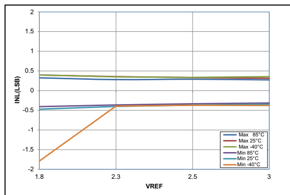
FIGURE 36-60: ADC 10-Bit Mode, Single-Ended INL, V_{DD} = 3.0V , T_{AD} = 1\text{ }\mu\text{S} (All devices)
