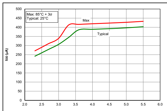
FIGURE 36-17: I_{DD} , XT Oscillator 4 MHz (PIC16F18326/46 only)
