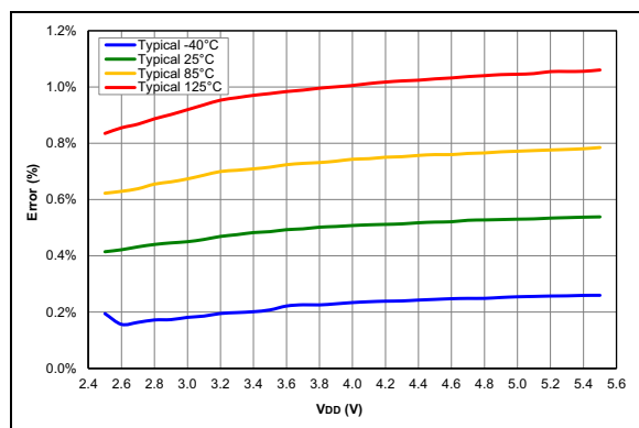
FIGURE 36-97: FVR Voltage Error 1x
