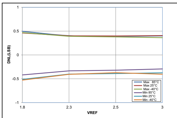
FIGURE 36-59: ADC 10-Bit Mode, Single-Ended DNL, V_{DD} = 3.0V , T_{AD} = 1\text{ }\mu\text{S} (All devices)
