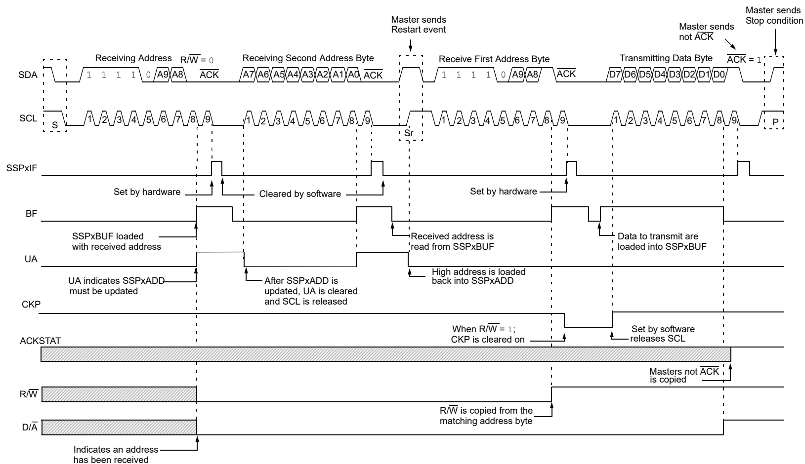
FIGURE 30-22: I 2 C SLAVE, 10-BIT ADDRESS, TRANSMISSION (SEN = 0, AHEN = 0, DHEN = 0)
