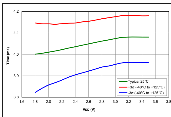
FIGURE 36-2: WDT Time-Out Period (PIC16LF18326/46 only)
