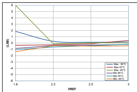
FIGURE 36-61: ADC 10-Bit Mode, Single-Ended Gain Error, V_{DD} = 3.0V , T_{AD} = 1\text{ }\mu s (All devices)
