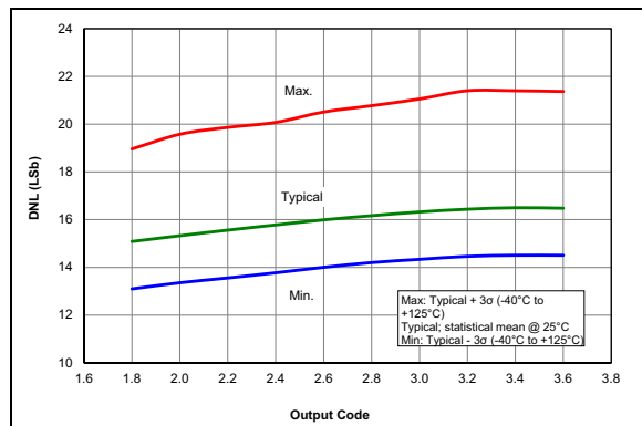
FIGURE 36-75: DAC INL Error, V_{DD} = 3.0V (PIC16LF18326/46 only)
