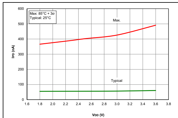
FIGURE 36-3: IPD Base, Low-Power Sleep Mode (PIC16LF18326/46 only)
