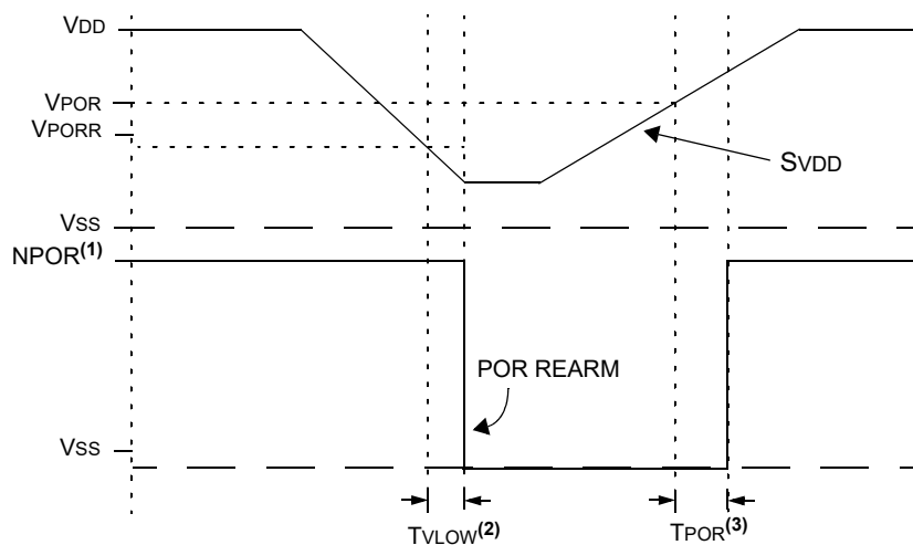
FIGURE 35-3: POR AND POR REARM WITH SLOW RISING V DD
