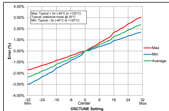
FIGURE 36-108: OSCUNE Center Frequency
