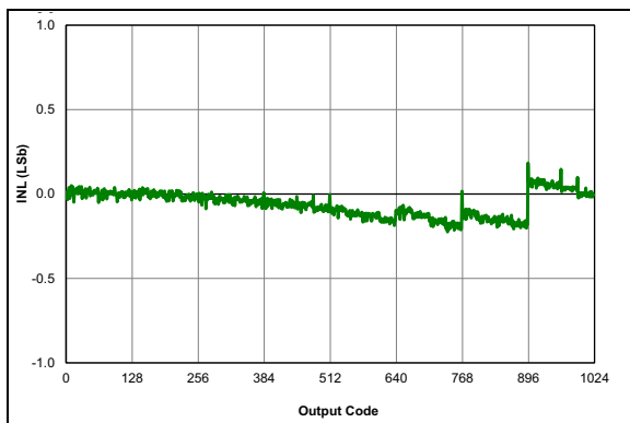
FIGURE 36-55: ADC 10-Bit Mode, Single-Ended INL, V_{DD} = 3.0V , V_{REF} = 3.0V , T_{AD} = 4\text{ }\mu\text{S} , 25^\circ\text{C} (All devices)
