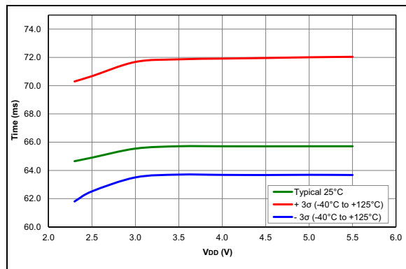
FIGURE 36-111: PWRT Period (PIC16F18326/46 only)
