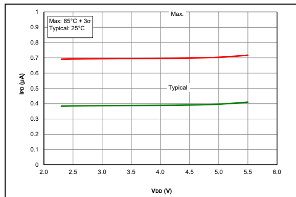
FIGURE 36-15: I_{PD} Base, 11 (PIC16F18326/46 only)
