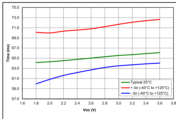
FIGURE 36-112: PWRT Period (PIC16LF18326/46 only)
