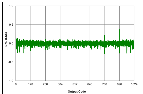
FIGURE 36-51: ADC 10-Bit Mode, Single-Ended DNL, V_{DD} = 3.0V , V_{REF} = 3.0V , T_{AD} = 1\text{ }\mu S , 25C (All devices)
