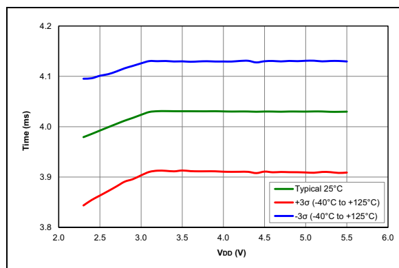
FIGURE 36-1: WDT Time-Out Period (PIC16F18326/46 only)
