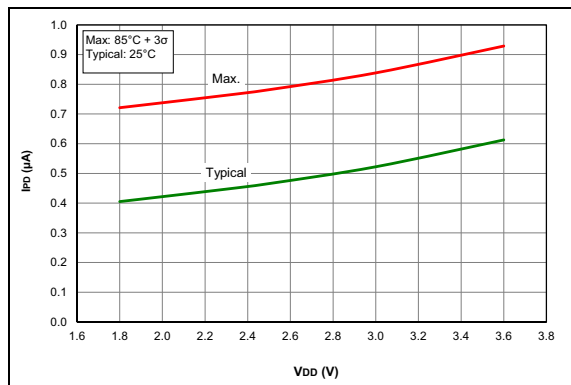
FIGURE 36-4: IPD, Watchdog Timer (WDT) (PIC16LF18326/46 only)
