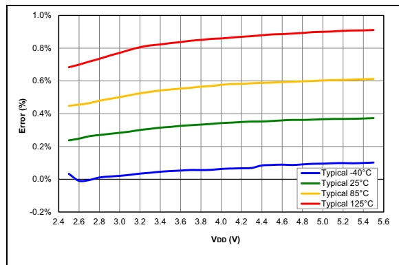
FIGURE 36-99: FVR Voltage Error 2x
