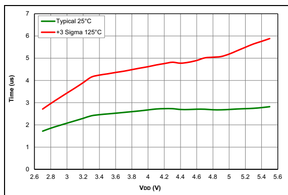
FIGURE 36-50: BOR Response Time (PIC16F18326/46 only)
