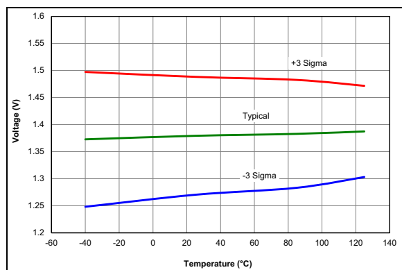
FIGURE 36-109: POR Release Voltage
