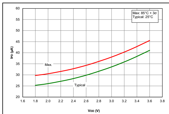
FIGURE 36-6: IPD, Fixed Voltage Reference (FVR) (PIC16LF18326/46 only)
