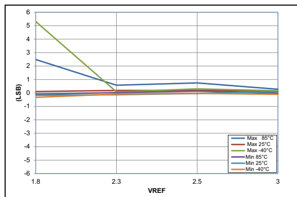
FIGURE 36-65: ADC 10-Bit Mode, Single-Ended Gain Error, V_{DD} = 3.0V , T_{AD} = 4\text{ }\mu s (All devices)
