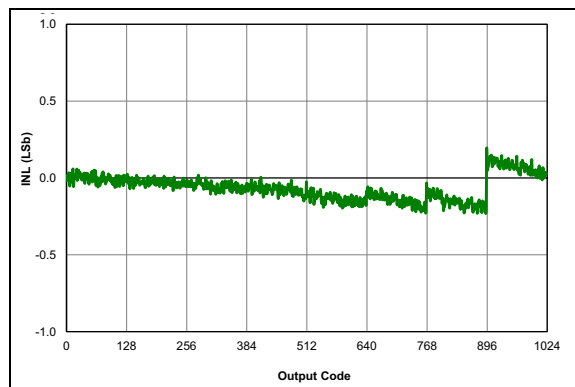
FIGURE 36-56: ADC 10-Bit Mode, Single-Ended INL, V_{DD} = 3.0V , V_{REF} = 3.0V , T_{AD} = 8\text{ }\mu\text{S} , 25^\circ\text{C} (All devices)
