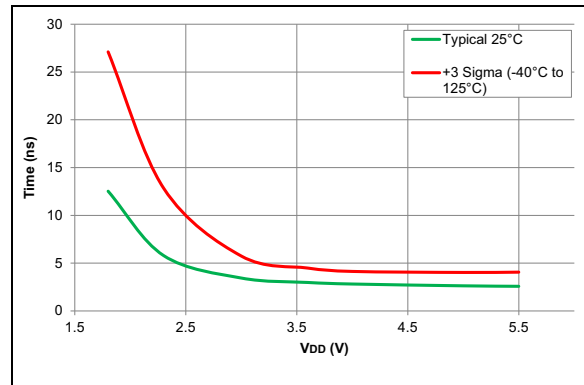
FIGURE 36-106: Rise Time, Slew Rate Control Disabled
