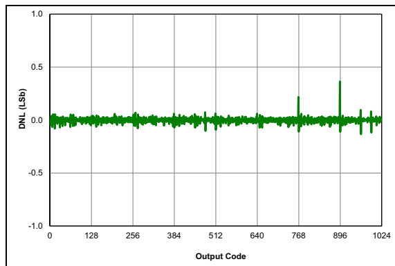
FIGURE 36-52: ADC 10-Bit Mode, Single-Ended DNL, V_{DD} = 3.0V , V_{REF} = 3.0V , T_{AD} = 4\text{ }\mu S , 25C (All devices)
