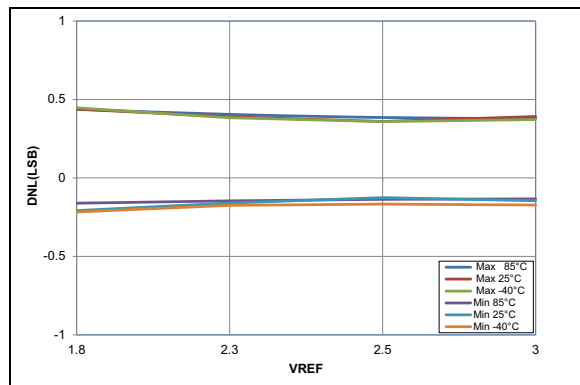
FIGURE 36-63: ADC 10-Bit Mode, Single-Ended DNL, V_{DD} = 3.0V , T_{AD} = 4\text{ }\mu s (All devices)
