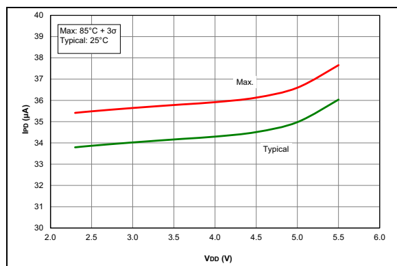
FIGURE 36-13: I_{PD} , Comparator (PIC16F18326/46 only)
