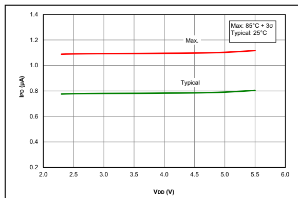
FIGURE 36-5: IPD, Watchdog Timer (WDT) (PIC16F18326/46 only)
