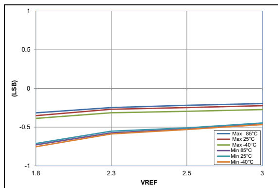
FIGURE 36-66: ADC 10-Bit Mode, Single-Ended Offset Error, V_{DD} = 3.0V , T_{AD} = 4\text{ }\mu s (All devices)
