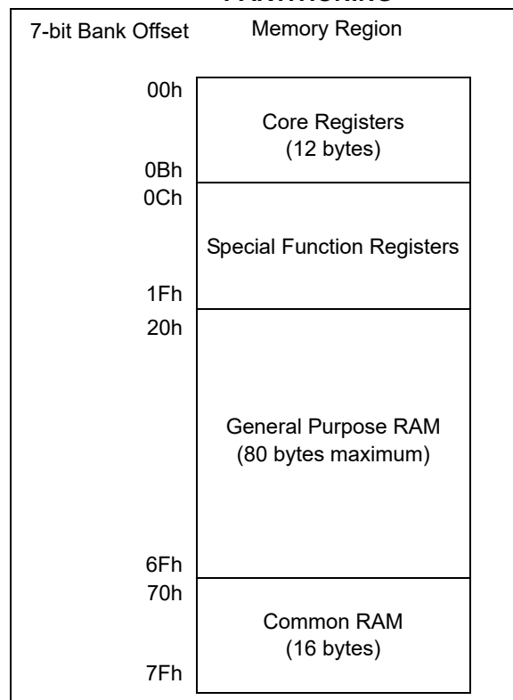
FIGURE 4-2: BANKED-MEMORY PARTITIONING
