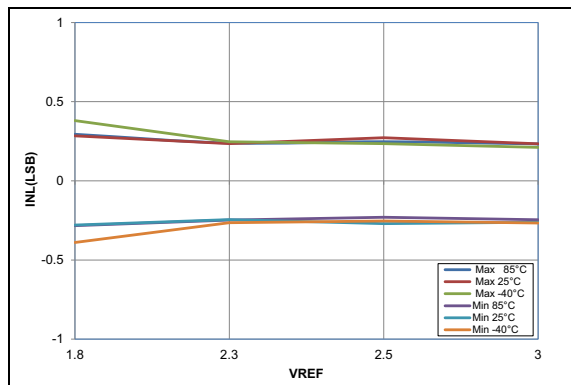
FIGURE 36-64: ADC 10-Bit Mode, Single-Ended INL, V_{DD} = 3.0V , T_{AD} = 4\text{ }\mu s (All devices)
