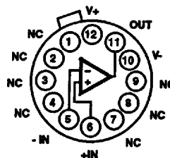
HA-5190/5195 (TO-8 METAL CAN) TOP VIEW
