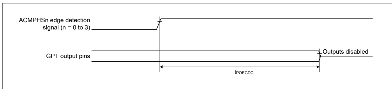
Figure 2.18 Output Disable Time for POEG in Response to Edge Detection Signal from ACPHPS
