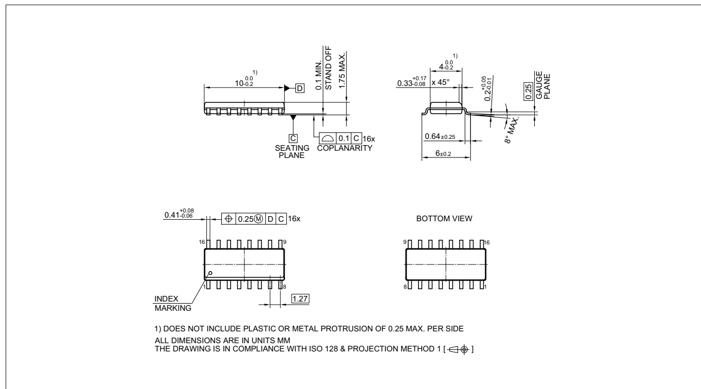
Figure 15 PG-DSO-16-11 outline
